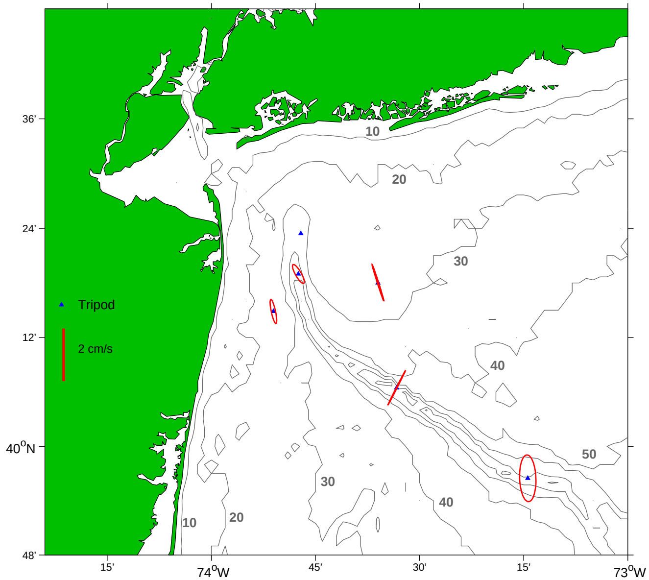
K_1 Tidal Ellipse, 15 mbs
