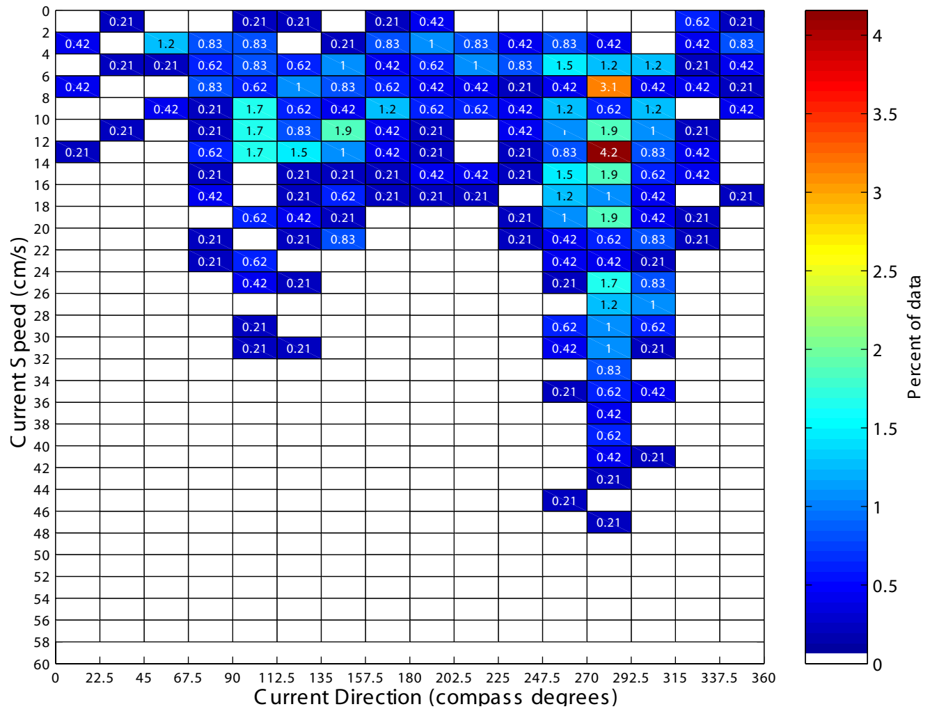
Station F: Sorted Current Speed and Direction for Low-Pass Filtered Data From ADCP* Sensor at Bottom (Depth = 70 m)
