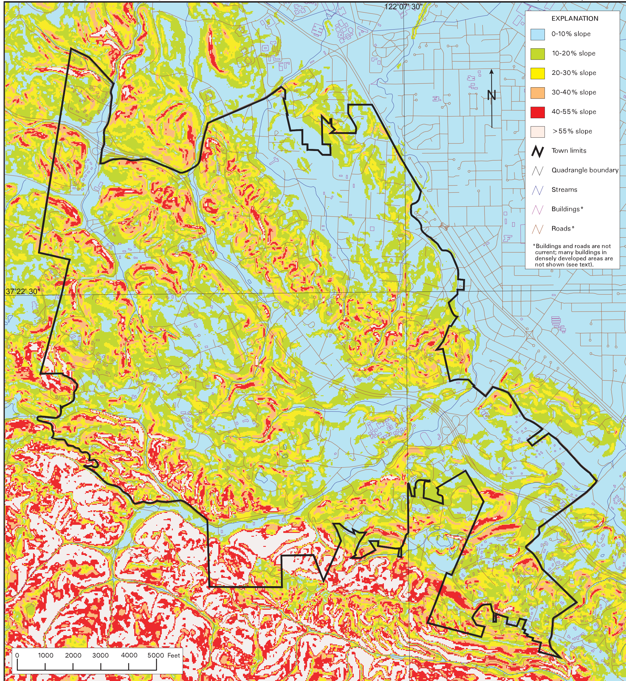
Figure 2. Slope Map of the Los Altos Hills Area, San Francisco Bay Area, California 1:24,000
