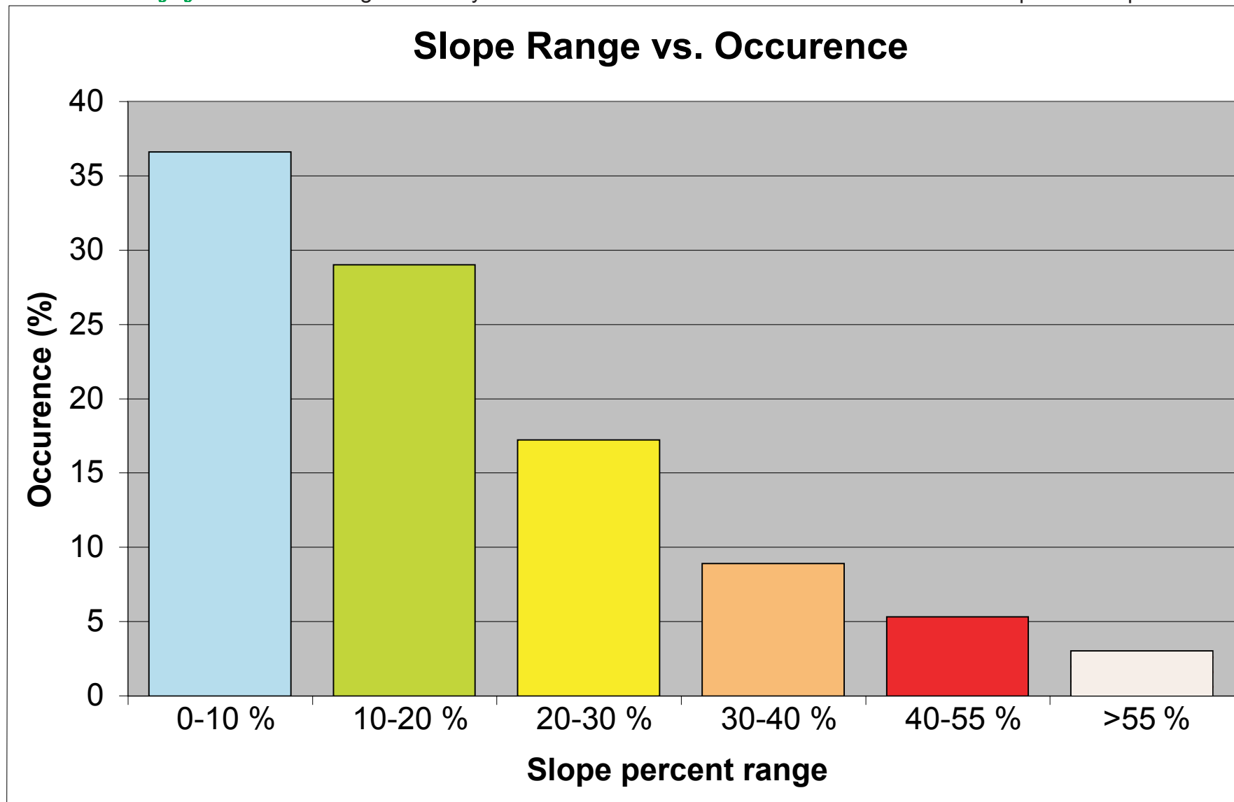
Figure 3. Histogram of Slope Range vs. Occurrence within the town limits of Los Altos Hills, San Francisco Bay Area, California
