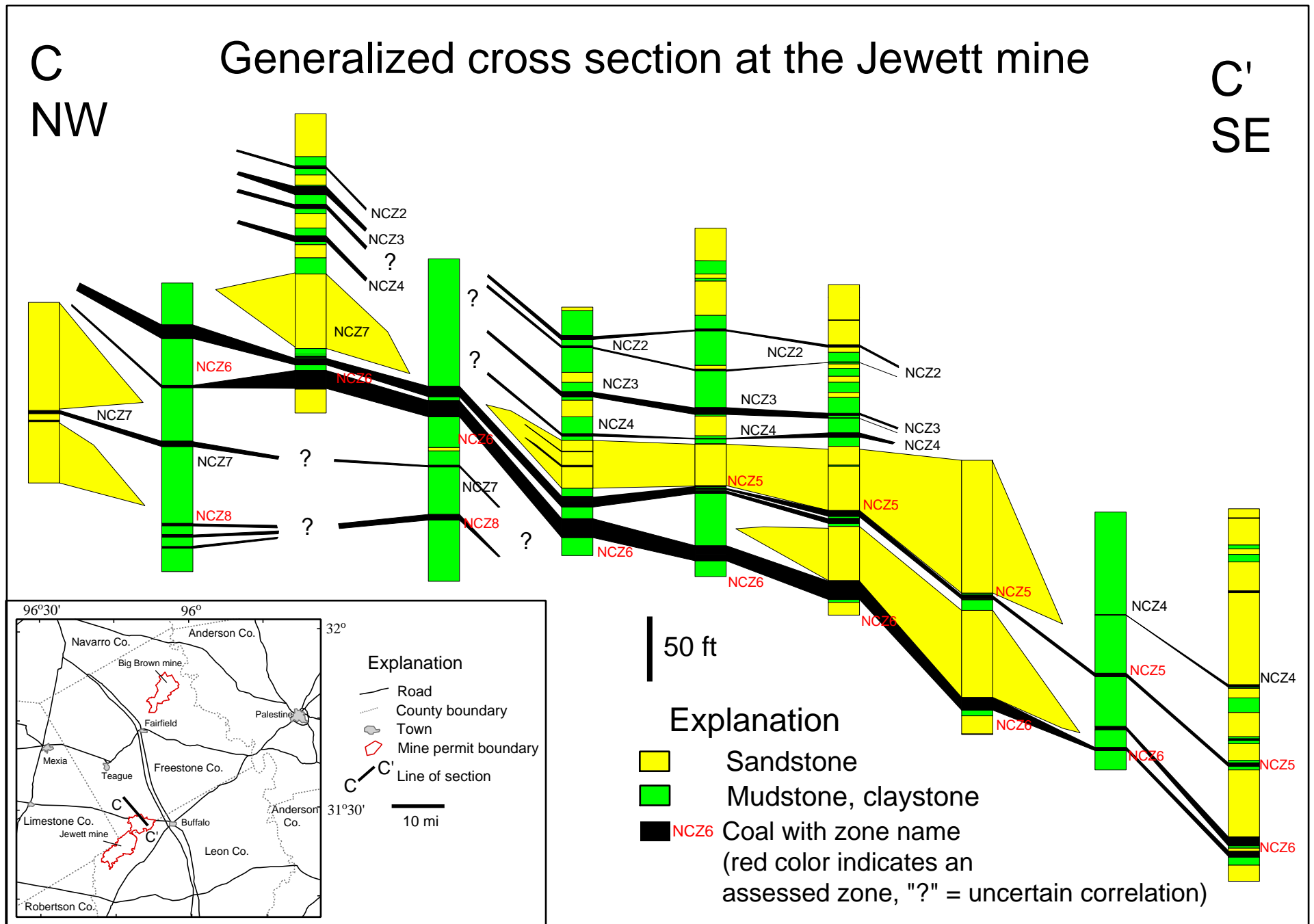
Fig. 6. Generalized cross section C-C' at the Jewett mine showing coal zone and lithologic variation. Coal zone names are shown in red and on figure 3 (only zones NCZ5, NCZ6, NCZ8, and NCZ9 were assessed). Inset map shows line of section.
