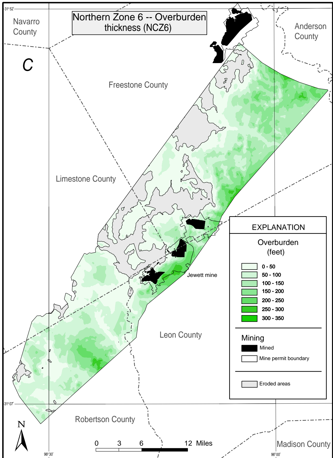
Fig. 10. Geology of northern Coal Zone 6 (NCZ6). a) Outline of Zone 6 showing coal mine permit locations mined areas, and county boundaries. b) Structure contour map of the stratigraphic top of Zone 6. c) Map of overburden thickness for Zone 6. d) Map of the cumulative coal bed thicknesses that compose Zone 6.
