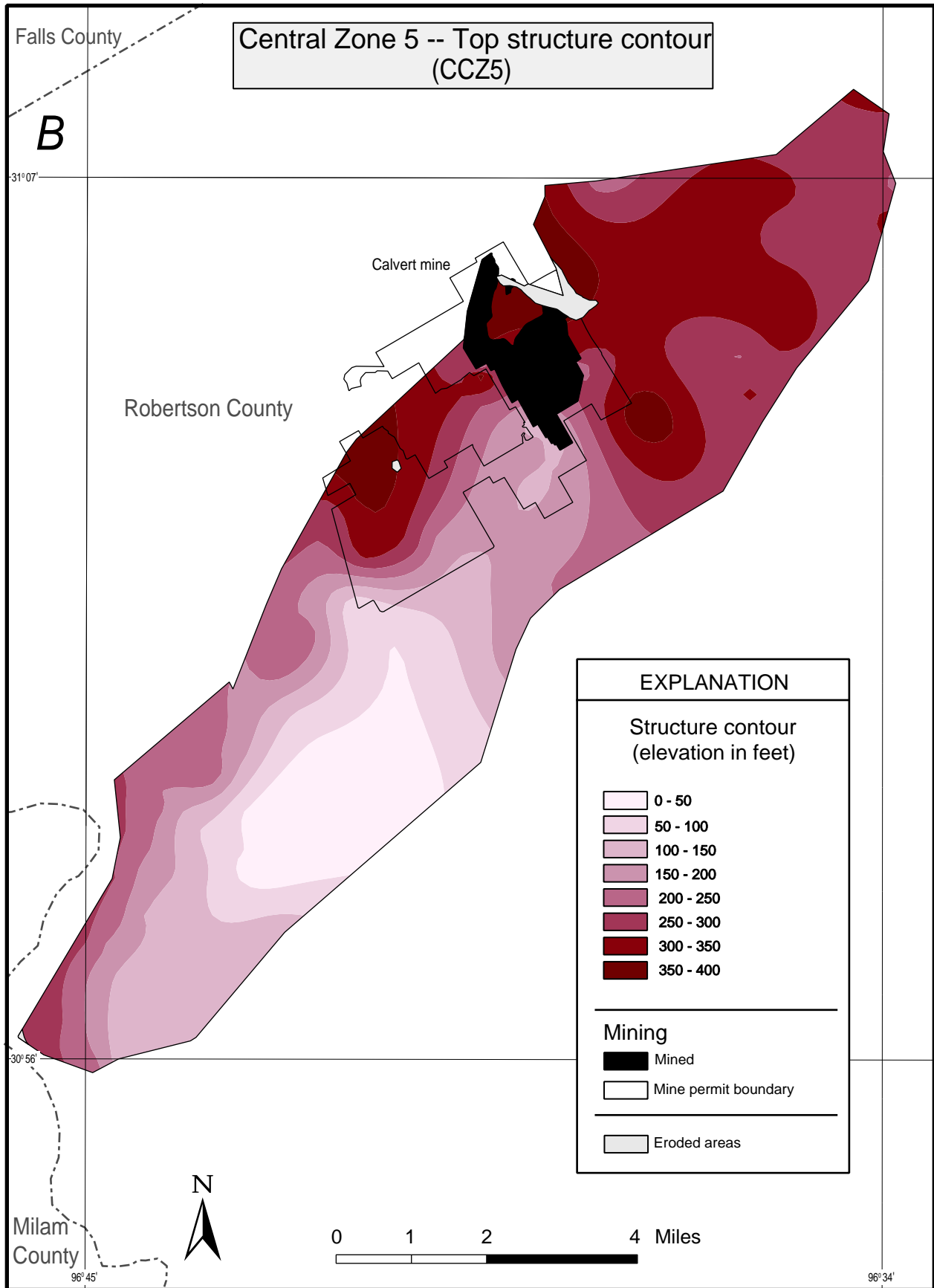
Fig. 14. Geology of central Coal Zone 5 (CCZ5). a) Outline of Zone 5 showing coal mine permit locations, mined areas, and county boundaries. b) Structure contour map of the stratigraphic top of Zone 5. c) Map of overburden thickness for Zone 5. d) Map of the cumulative coal bed thicknesses that compose Zone 5.
