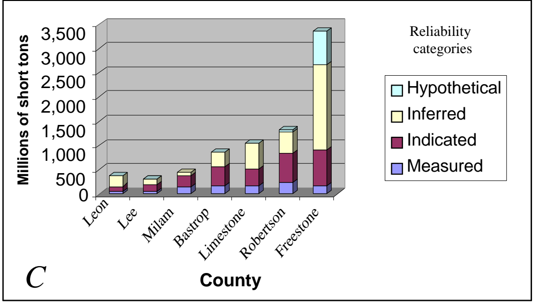
Fig. 18. Coal resources for the central Texas study area by county and a) overburden thickness, b) coal zone thickness, and c) reliability categories. Coal resources for the central Texas study area are also plotted by zone and d) overburden thickness, e) coal zone thickness, and f) reliability categories.
