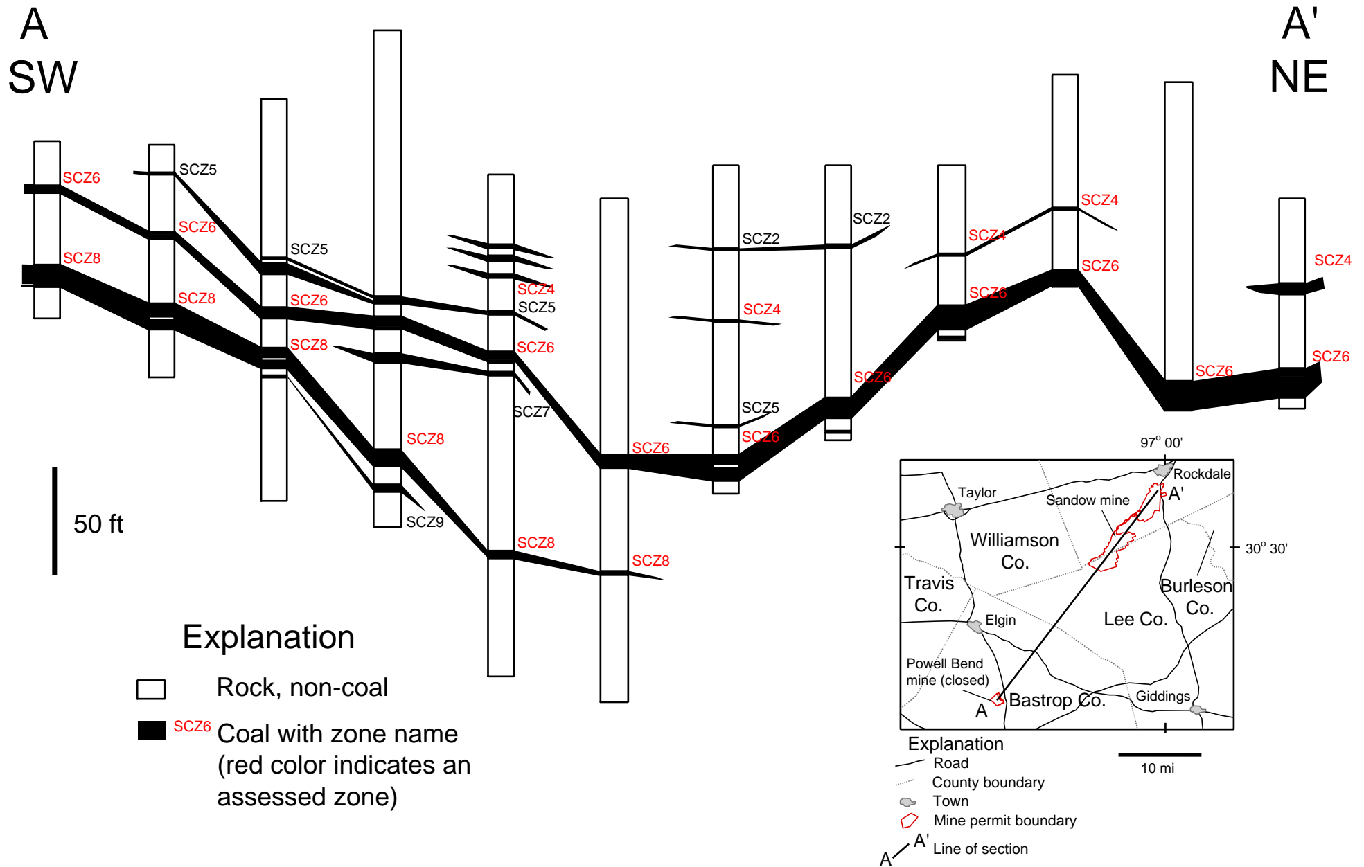
Fig. 4. Generalized cross section A-A' through the Powell Bend and Sandow mines showing correlation and variation of coal zones. Coal zone names are shown in red and on figure 3 (only zones SCZ4, SCZ6, and SCZ8 were assessed). Inset map shows line of section.
