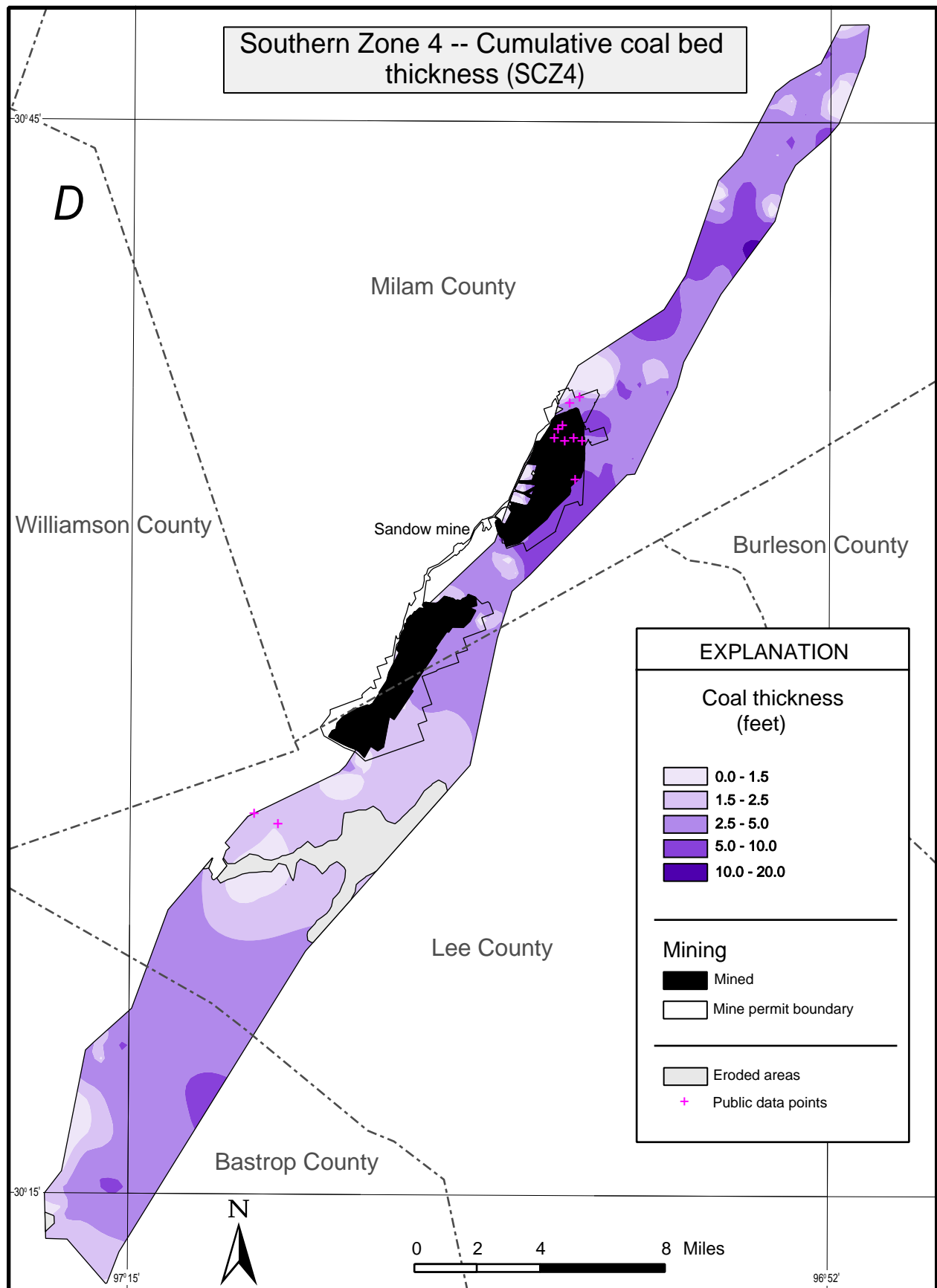
Fig. 15. Geology of southern Coal Zone 4 (SCZ4). a) Outline of Zone 4 showing coal mine permit locations, mined areas, and county boundaries. b) Structure contour map of the stratigraphic top of Zone 4. c) Map of overburden thickness for Zone 4. d) Map of the cumulative coal bed thicknesses that compose Zone 4.
