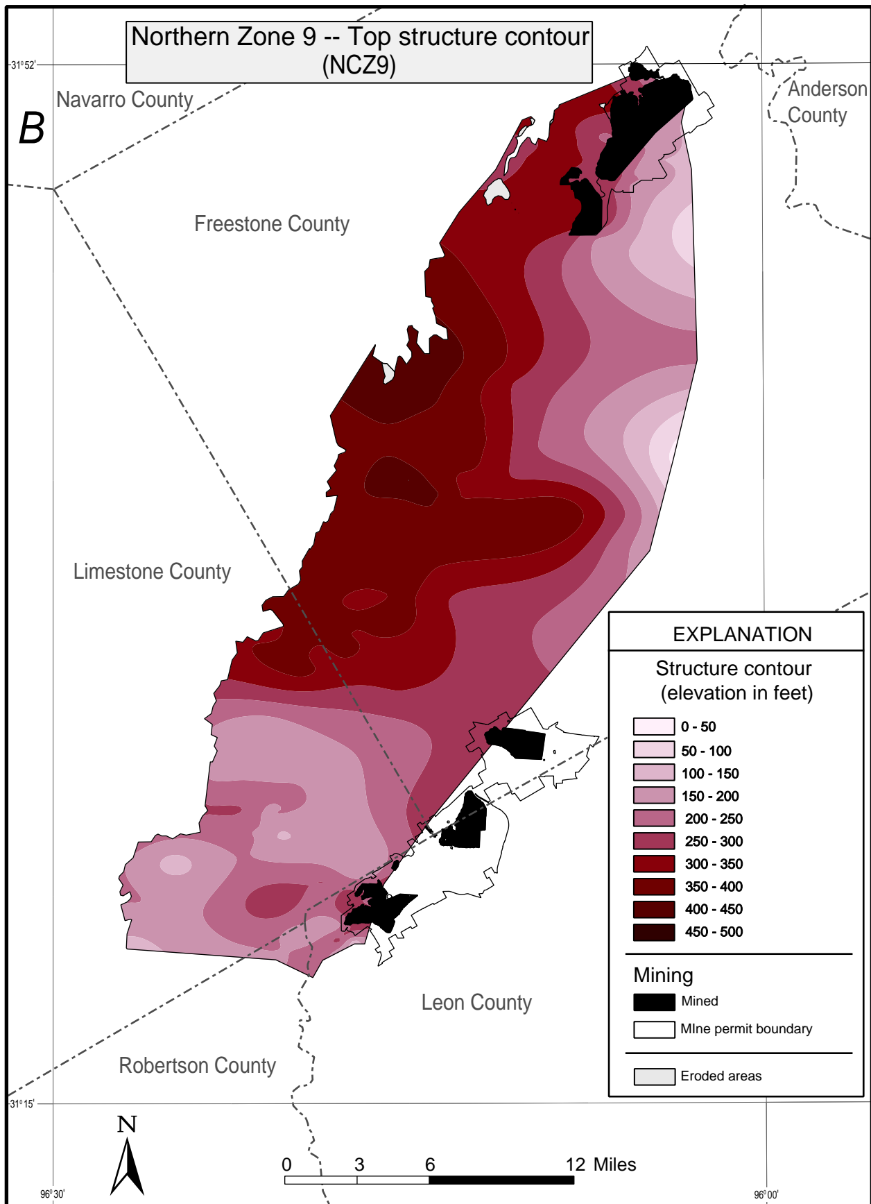
Fig. 12. Geology of northern Coal Zone 9 (NCZ9). a) Outline of Zone 9 showing coal mine permit locations mined areas, and county boundaries. b) Structure contour map of the stratigraphic top of Zone 9. c) Map of overburden thickness for Zone 9. d) Map of the cumulative coal bed thicknesses that compose Zone 9.
