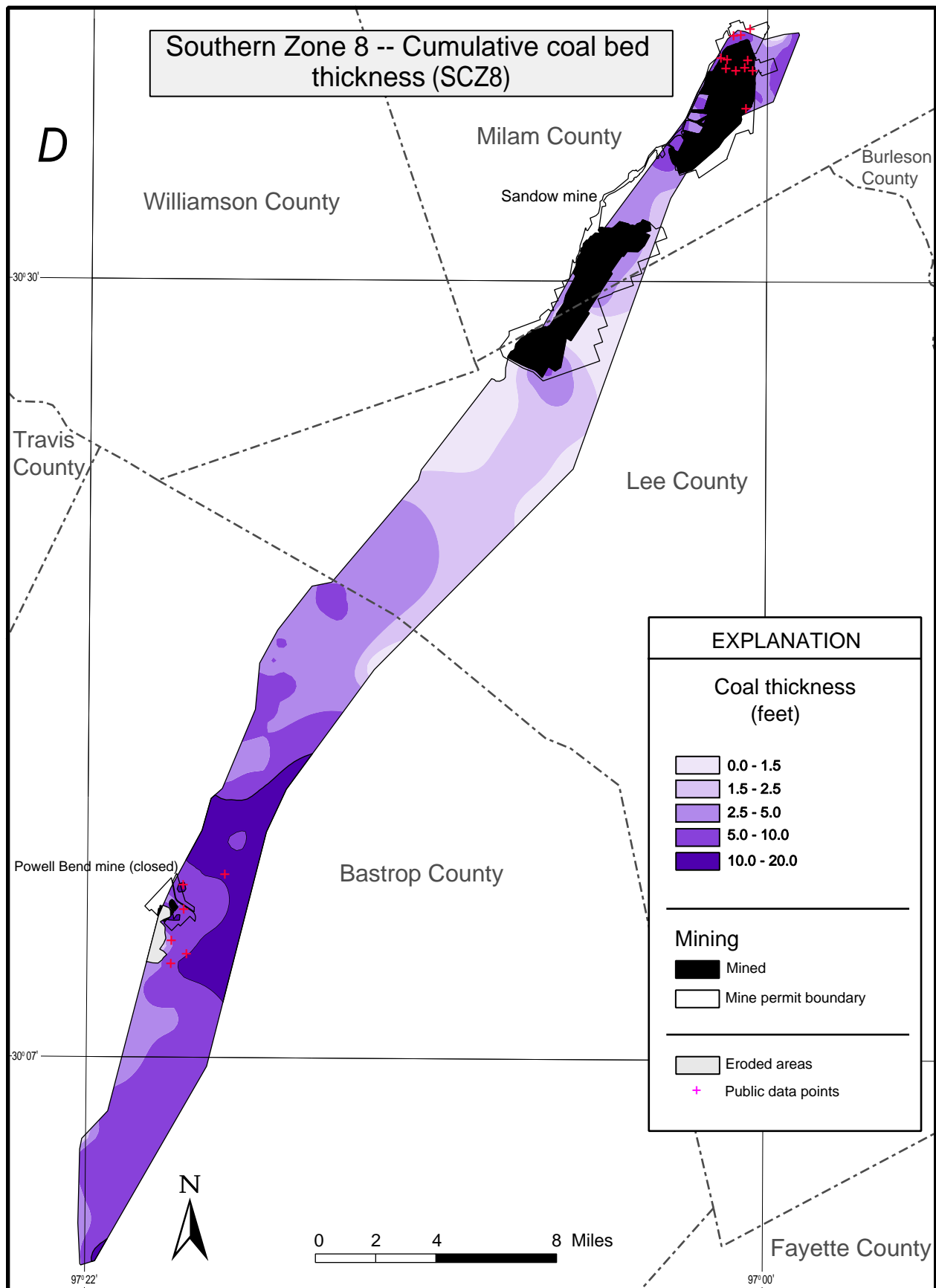
Fig. 17. Geology of southern Coal Zone 8 (SCZ8). a) Outline of Zone 8 showing coal mine permit locations, mined areas, and county boundaries. b) Structure contour map of the stratigraphic top of Zone 8. c) Map of overburden thickness for Zone 8. d) Map of the cumulative coal bed thicknesses that compose Zone 8.
