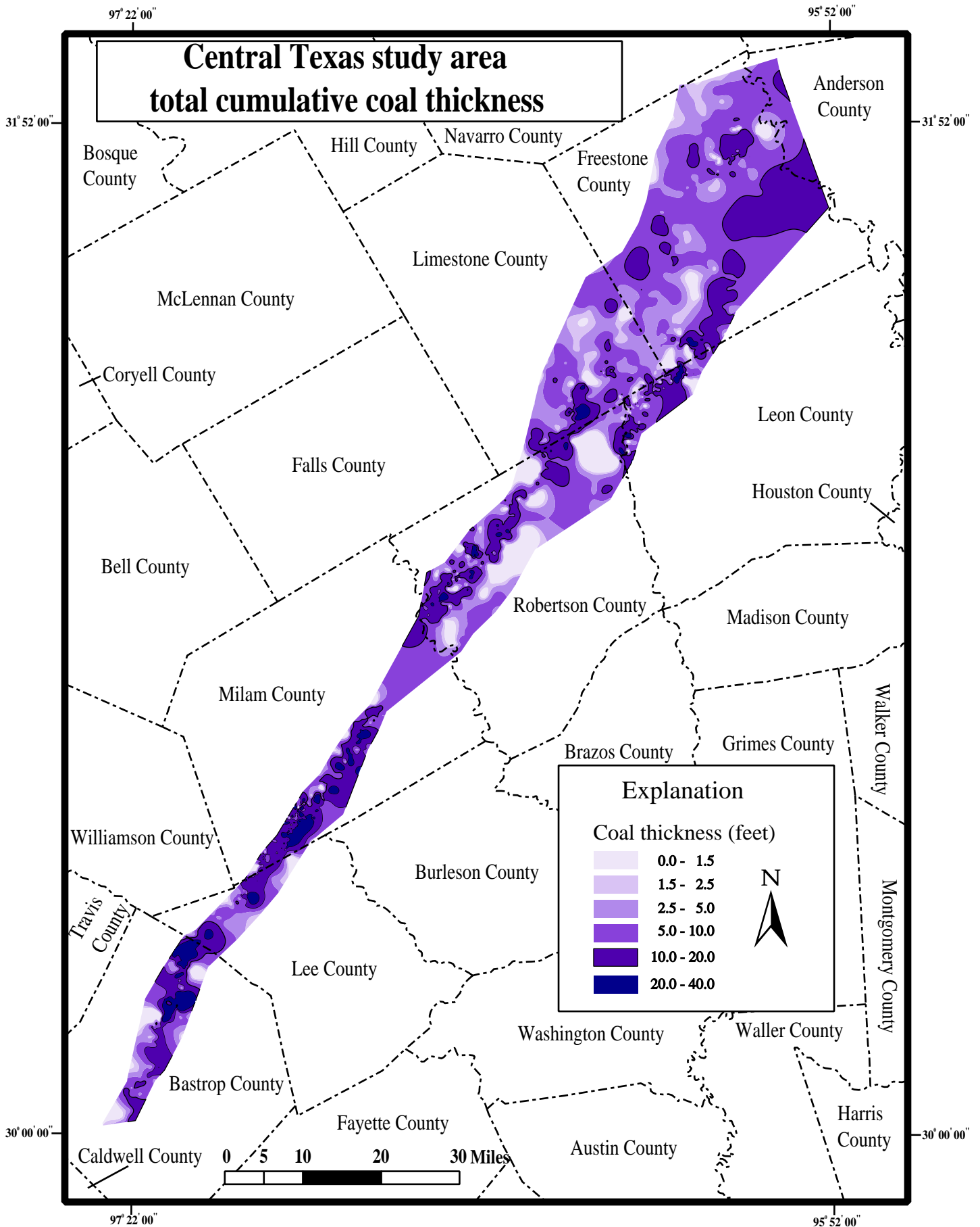
Fig. 19. Map of the total cumulative coal resources for the central Texas study area.
