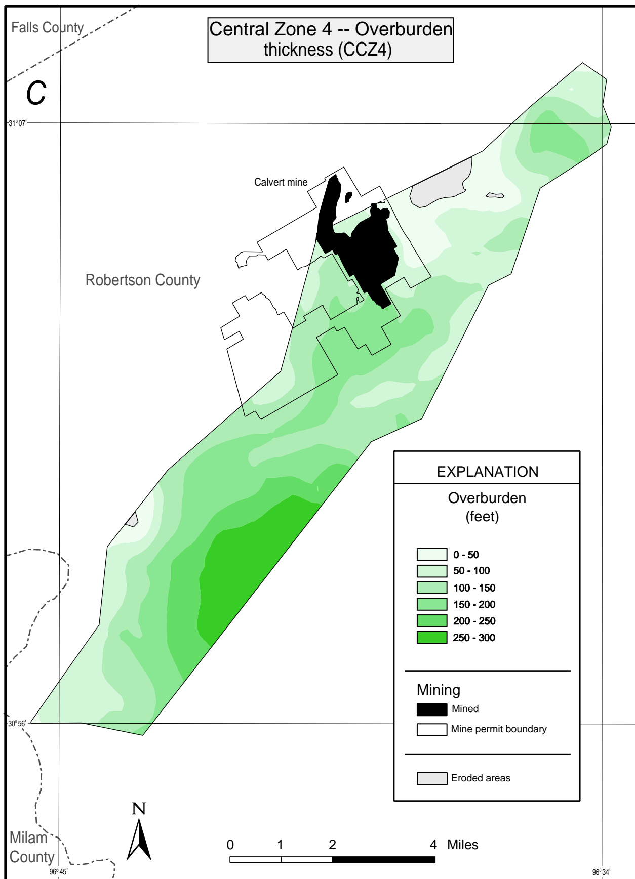
Fig. 13. Geology of central Coal Zone 4 (CCZ4). a) Outline of Zone 4 showing coal mine permit locations mined areas, and county boundaries. b) Structure contour map of the stratigraphic top of Zone 4. c) Map of overburden thickness for Zone 4. d) Map of the cumulative coal bed thicknesses that compose Zone 4.
