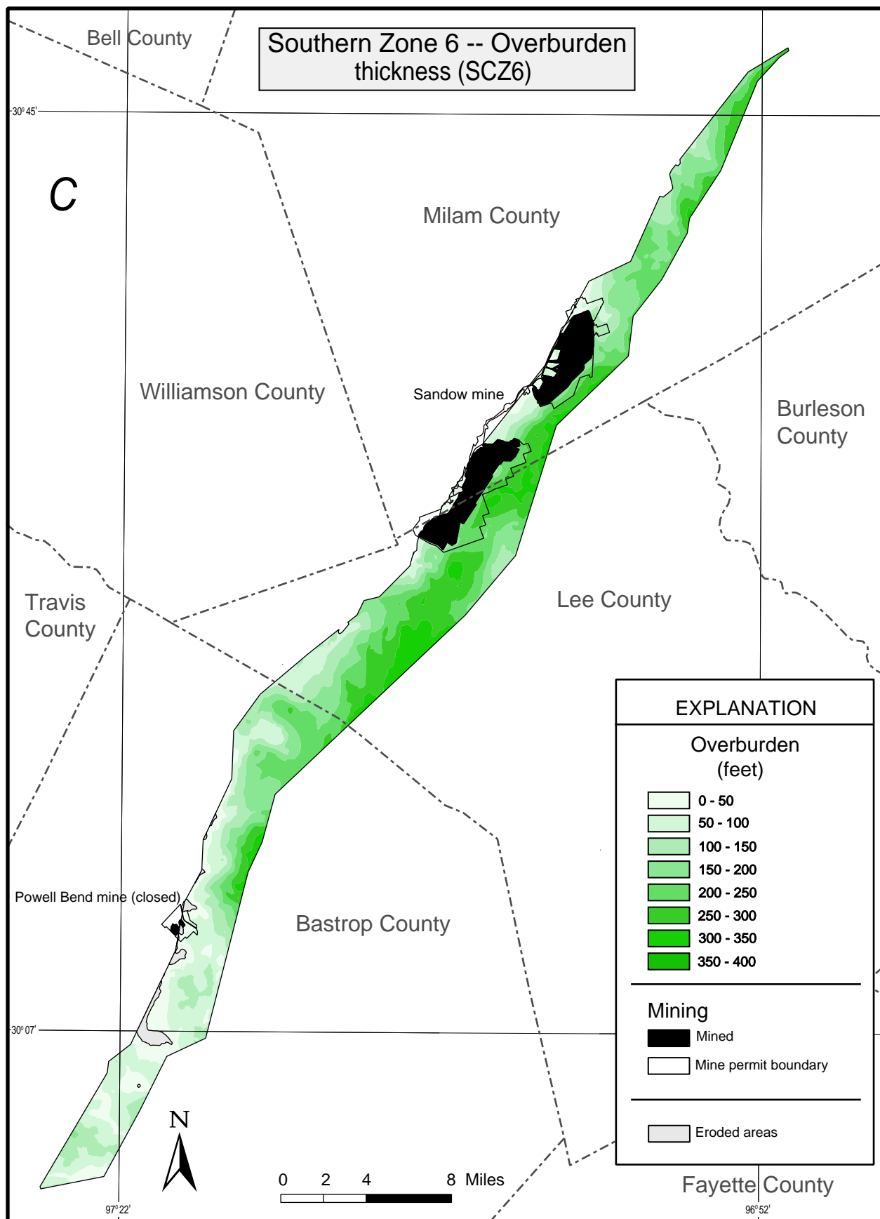
Fig. 16. Geology of southern Coal Zone 6 (SCZ6). a) Outline of Zone 6 showing coal mine locations, mined areas, and county boundaries. b) Structure contour map of the stratigraphic top of Zone 6. c) Map of overburden thickness for Zone 6. d) Map of the cumulative coal bed thicknesses that compose Zone 6.
