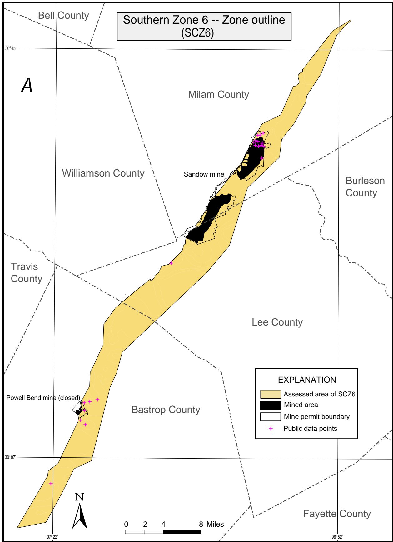
Fig. 16. Geology of southern Coal Zone 6 (SCZ6). a) Outline of Zone 6 showing coal mine locations, mined areas, and county boundaries. b) Structure contour map of the stratigraphic top of Zone 6. c) Map of overburden thickness for Zone 6. d) Map of the cumulative coal bed thicknesses that compose Zone 6.
