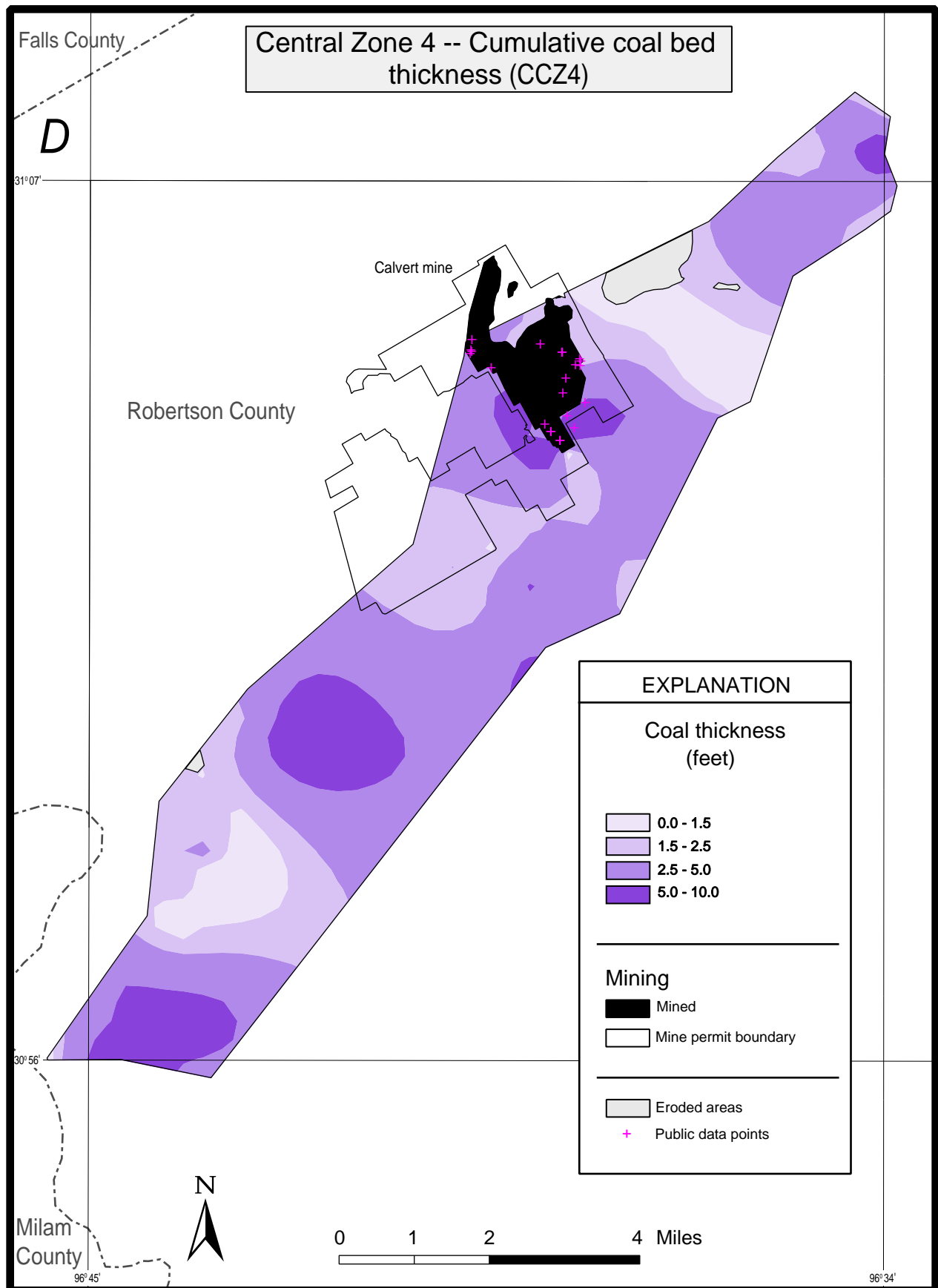
Fig. 13. Geology of central Coal Zone 4 (CCZ4). a) Outline of Zone 4 showing coal mine permit locations mined areas, and county boundaries. b) Structure contour map of the stratigraphic top of Zone 4. c) Map of overburden thickness for Zone 4. d) Map of the cumulative coal bed thicknesses that compose Zone 4.
