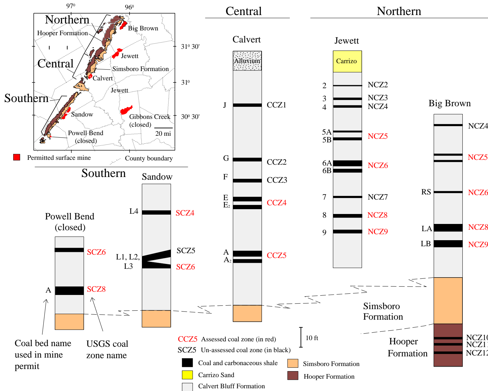
Fig. 3. Generalized stratigraphic sections of Wilcox strata in the central Texas study area showing the stratigraphic position of coal zones and names used in this study. Locations of mines are shown on the inset map and figure 2. Coal zone names used in this study are prefixed by "N" for northern resource areas; "C" for the central resource areas; "S" for the southern resource areas, and "CZ" for coal zone, are shown on the right of each stratigraphic section and generally follow the names used at the Jewett mine (Palmquist, 1987; Jewett mine permit applications on file at the Railroad Commission of Texas, Surface Mining and Reclamation Division, in Austin, Texas). Stratigraphic bed and zone names used in mine permits other than the Jewett mine are shown on the left of each stratigraphic section and are found in the various mine permit applications on file at the Railroad Commission of Texas, Surface Mining and Reclamation Division, in Austin, Texas (table 1).
