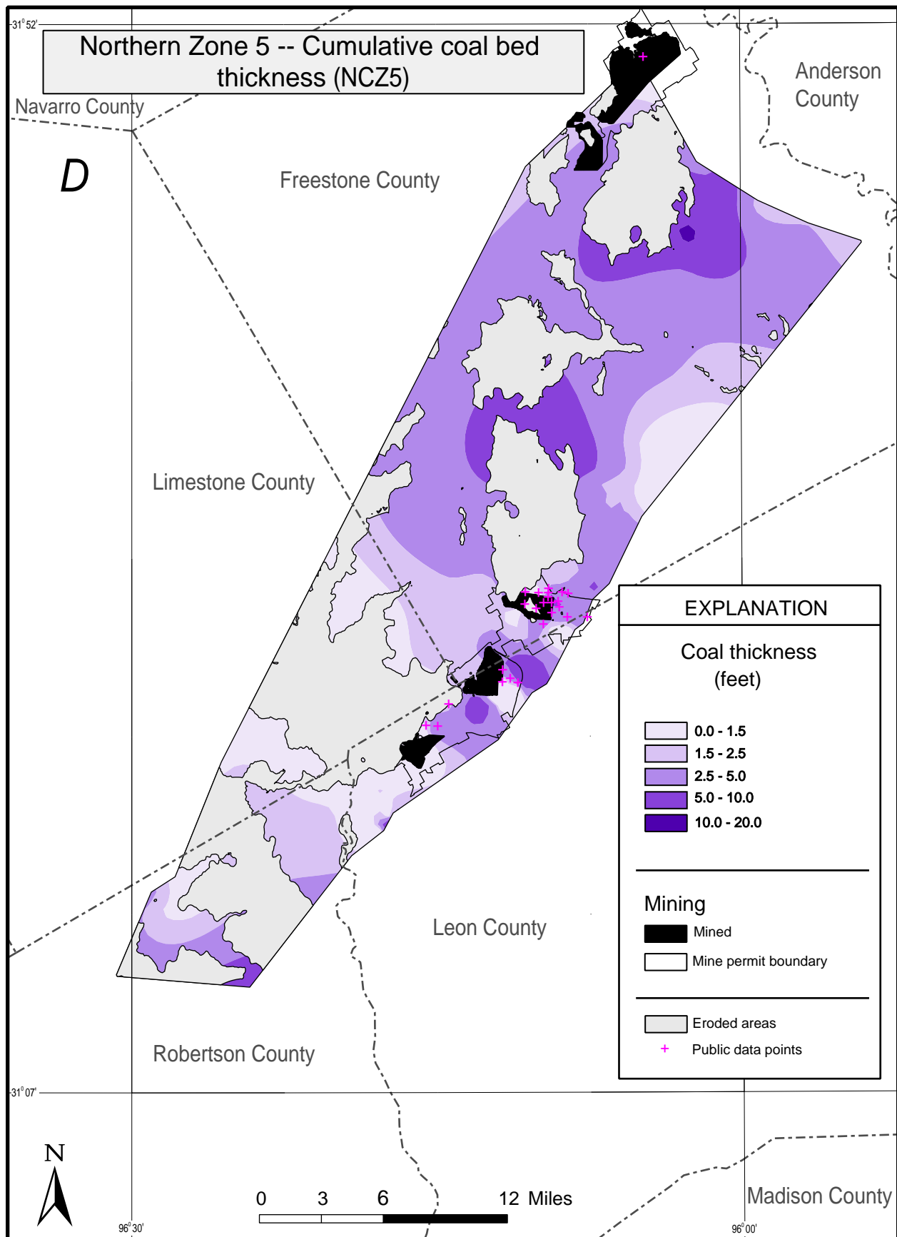
Fig. 9. Geology of northern Coal Zone 5 (NCZ5) of central Texas. a) Outline of Zone 5 showing coal mine permit locations, mined areas, and county boundaries. b) Structure contour map of the stratigraphic top of Zone 5. c) Map of overburden thickness for Zone 5. d) Map of the cumulative coal bed thicknesses that compose Zone 5.
