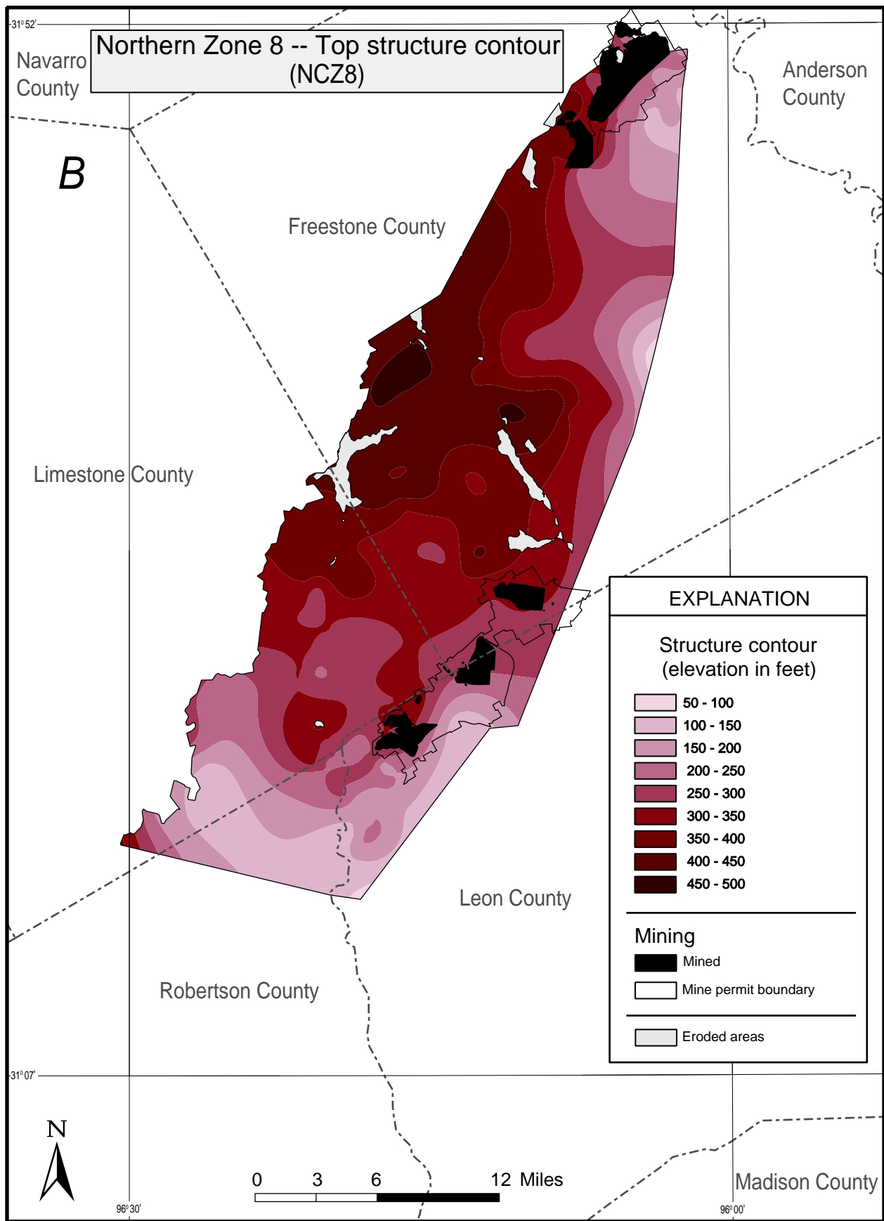
Fig. 11. Geology of coal northern Coal Zone 8 (NCZ8). a) Outline of Zone 8 showing coal mine permit locations mined areas, and county boundaries. b) Structure contour map of the stratigraphic top of Zone 8. c) Map of overburden thickness for Zone 8. d) Map of the cumulative coal bed thicknesses that compose Zone 8.
