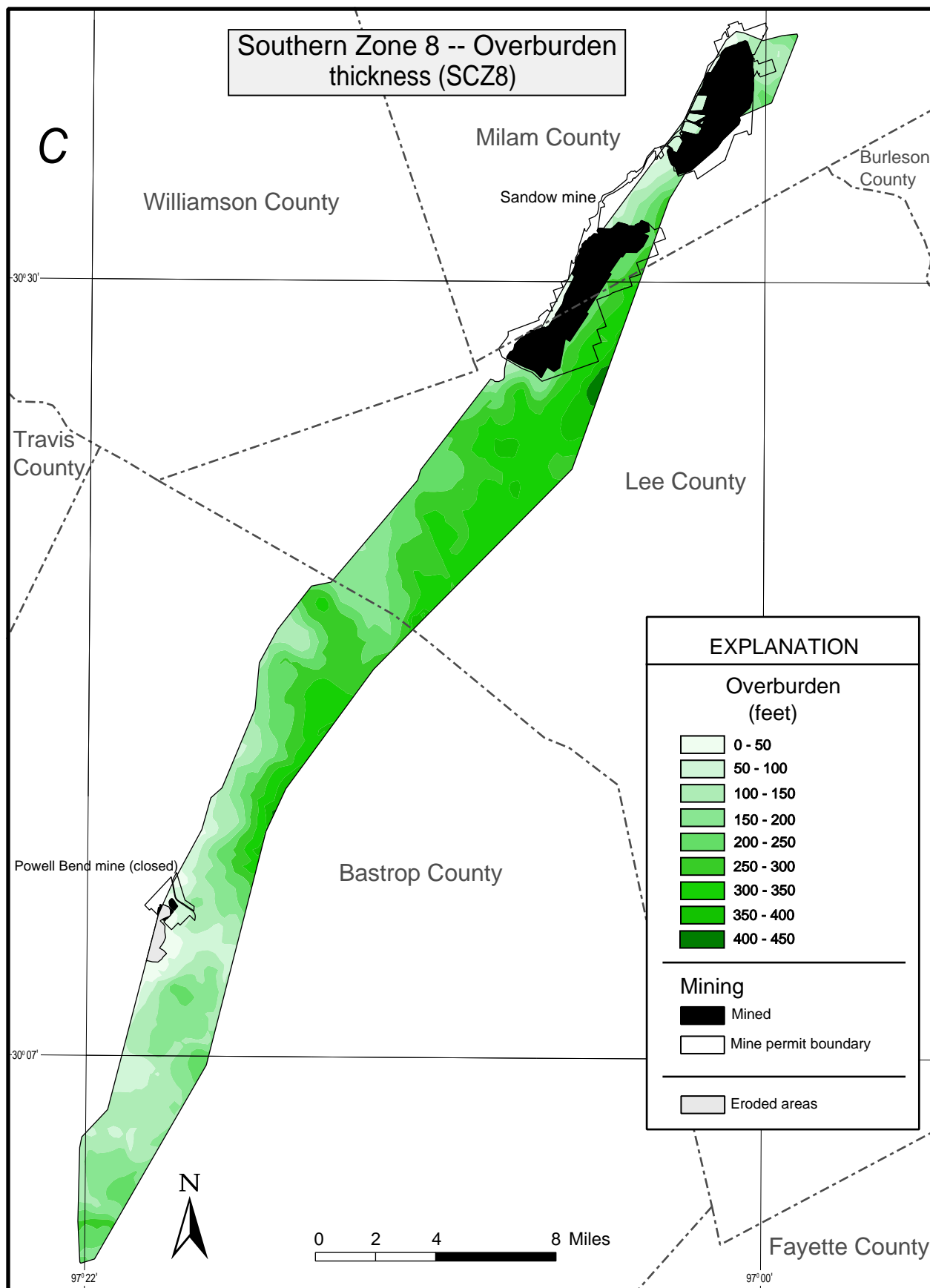
Fig. 17. Geology of southern Coal Zone 8 (SCZ8). a) Outline of Zone 8 showing coal mine permit locations, mined areas, and county boundaries. b) Structure contour map of the stratigraphic top of Zone 8. c) Map of overburden thickness for Zone 8. d) Map of the cumulative coal bed thicknesses that compose Zone 8.
