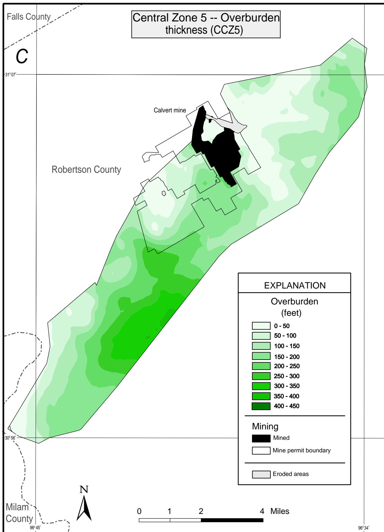
Fig. 14. Geology of central Coal Zone 5 (CCZ5). a) Outline of Zone 5 showing coal mine permit locations, mined areas, and county boundaries. b) Structure contour map of the stratigraphic top of Zone 5. c) Map of overburden thickness for Zone 5. d) Map of the cumulative coal bed thicknesses that compose Zone 5.
