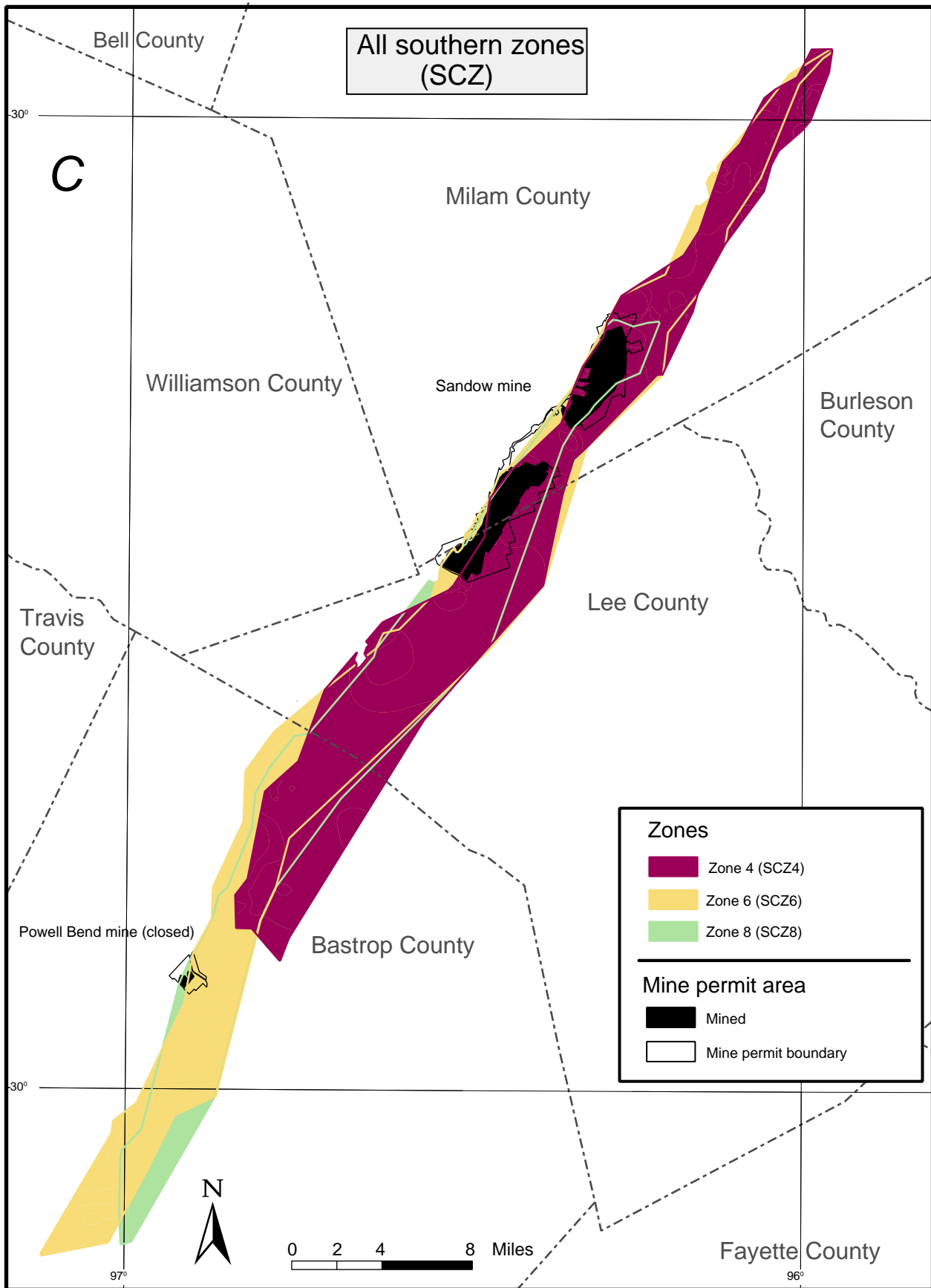
Fig. 8. Regional extent of the nine coal zones evaluated for resources in study of the coal resources in central Texas. The extent of individual assessment units is limited by up-dip outcrop and data availability. a) Northern coal zones; b) central coal zones; and c) southern coal zones.
