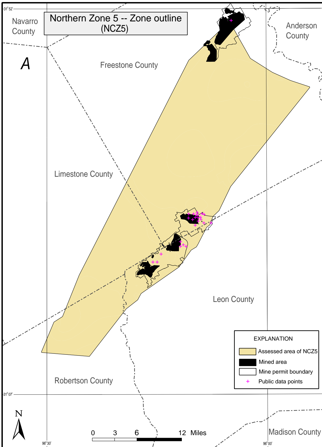
Fig. 9. Geology of northern Coal Zone 5 (NCZ5) of central Texas. a) Outline of Zone 5 showing coal mine permit locations, mined areas, and county boundaries. b) Structure contour map of the stratigraphic top of Zone 5. c) Map of overburden thickness for Zone 5. d) Map of the cumulative coal bed thicknesses that compose Zone 5.
