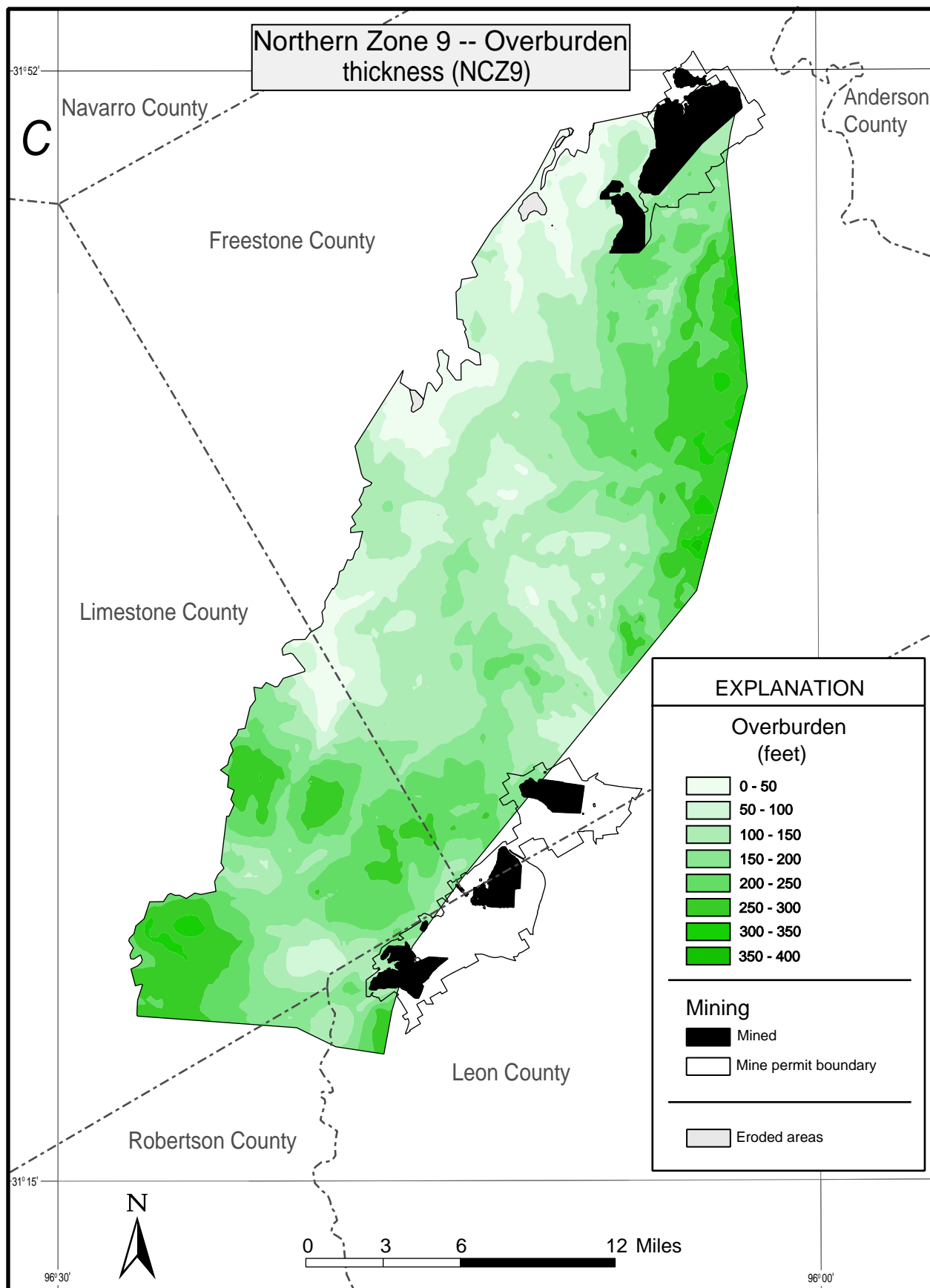
Fig. 12. Geology of northern Coal Zone 9 (NCZ9). a) Outline of Zone 9 showing coal mine permit locations mined areas, and county boundaries. b) Structure contour map of the stratigraphic top of Zone 9. c) Map of overburden thickness for Zone 9. d) Map of the cumulative coal bed thicknesses that compose Zone 9.
