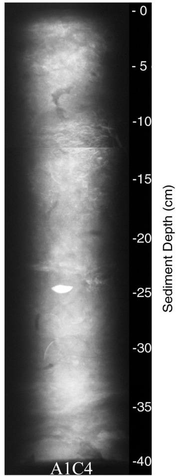
Core A1C4 was taken on June 18, 1996 in 9 meters of water. The core measured 41 cm in length and was x-rayed on July 1, 1996. Features noted are seen in the x-ray above and include mottled sediment, wispy sand and mud deposits, and some biological features such as small shells.
