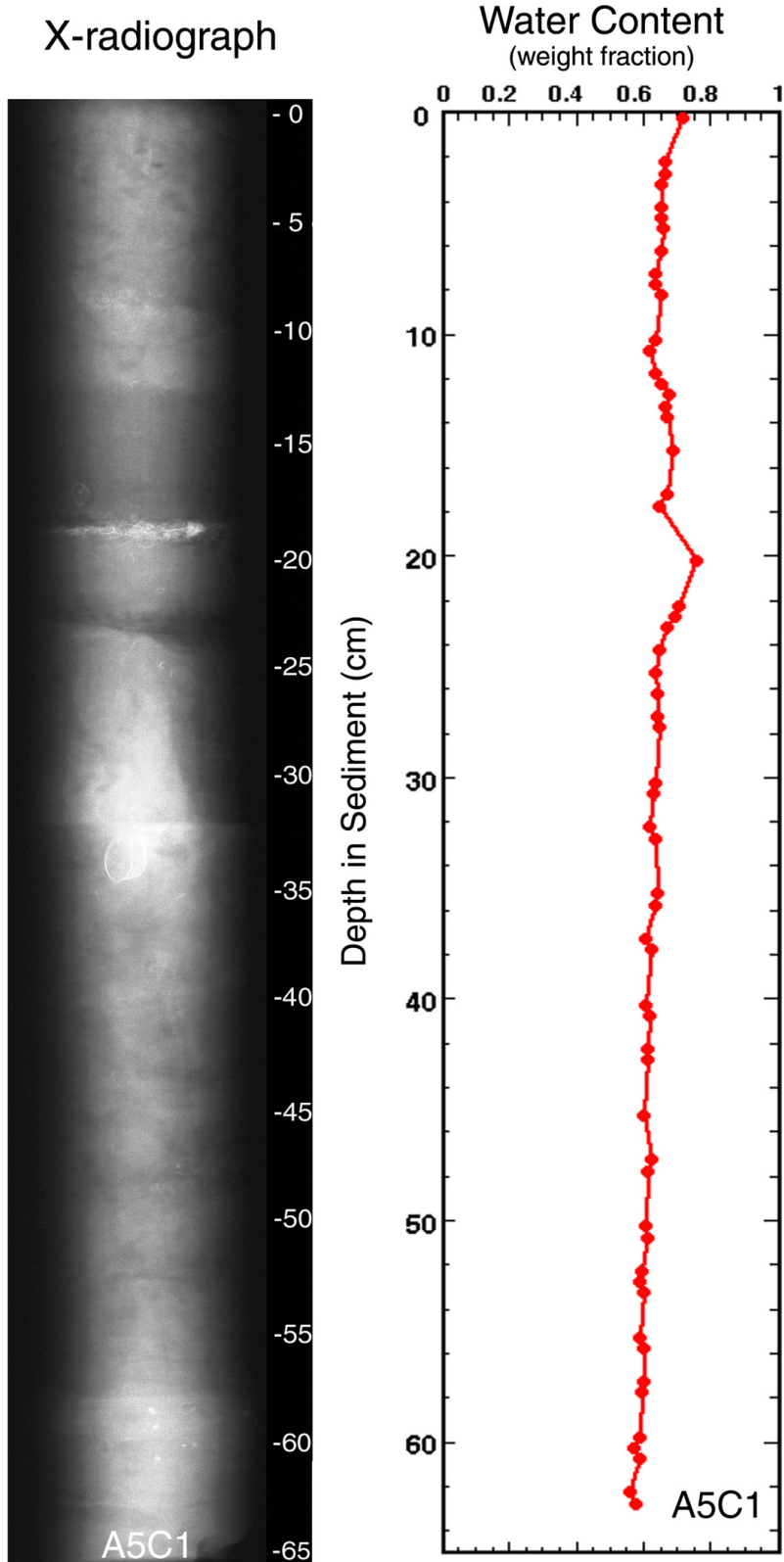
Core A5C1 was taken on June 18, 1996 in 28 meters of water. The core measured 65 cm in length, was x-rayed on June 26, 1996 and was subsampled on May 13, 1997 at 0.5 cm intervals down the whole core. Features noted are seen in the x-ray and water content profiles above and include mottled sediment, mud and sand deposits, and some biological features such as small shells, including a shell layer visible at ~18 cm down core. No textural analysis is intended for this core.
