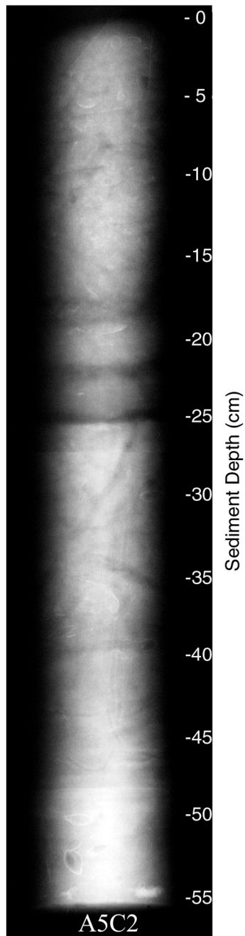
Core A5C2 was taken on June 18, 1996 in 28 meters of water. The core measured 56 cm in length and was x-rayed on June 26, 1996. Features noted are seen in the x-ray profile above and include mud and sand ribbons, some slightly mottled sediment, rocks, and biological features including worm tubes and small shells.
