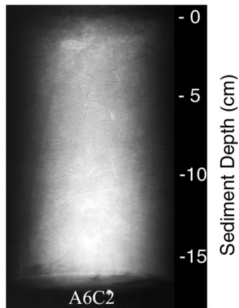
Core A6C2 was taken on June 18, 1996 in 19 meters of water. The core measured 16.5 cm in length and was x-rayed on July 2, 1996. This core was frozen during the x-radiograph and ice crystals are visible in the x-ray image. Features noted are seen in the x-ray profile above and include mottled sediment and some biological features such as shells and worm tubes.
