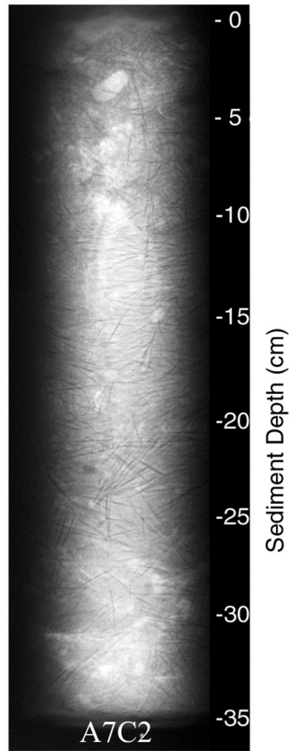
Core A7C2 was taken on June 18, 1996 in 15 meters of water. The core measured 35 cm in length, and was x-rayed on June 26, 1996. The core was frozen during the x-radiograph and ice crystals are visible in the x-ray image. Features noted are seen in the x-ray profile above and include mottled sediment, rocks, and some biological features.
