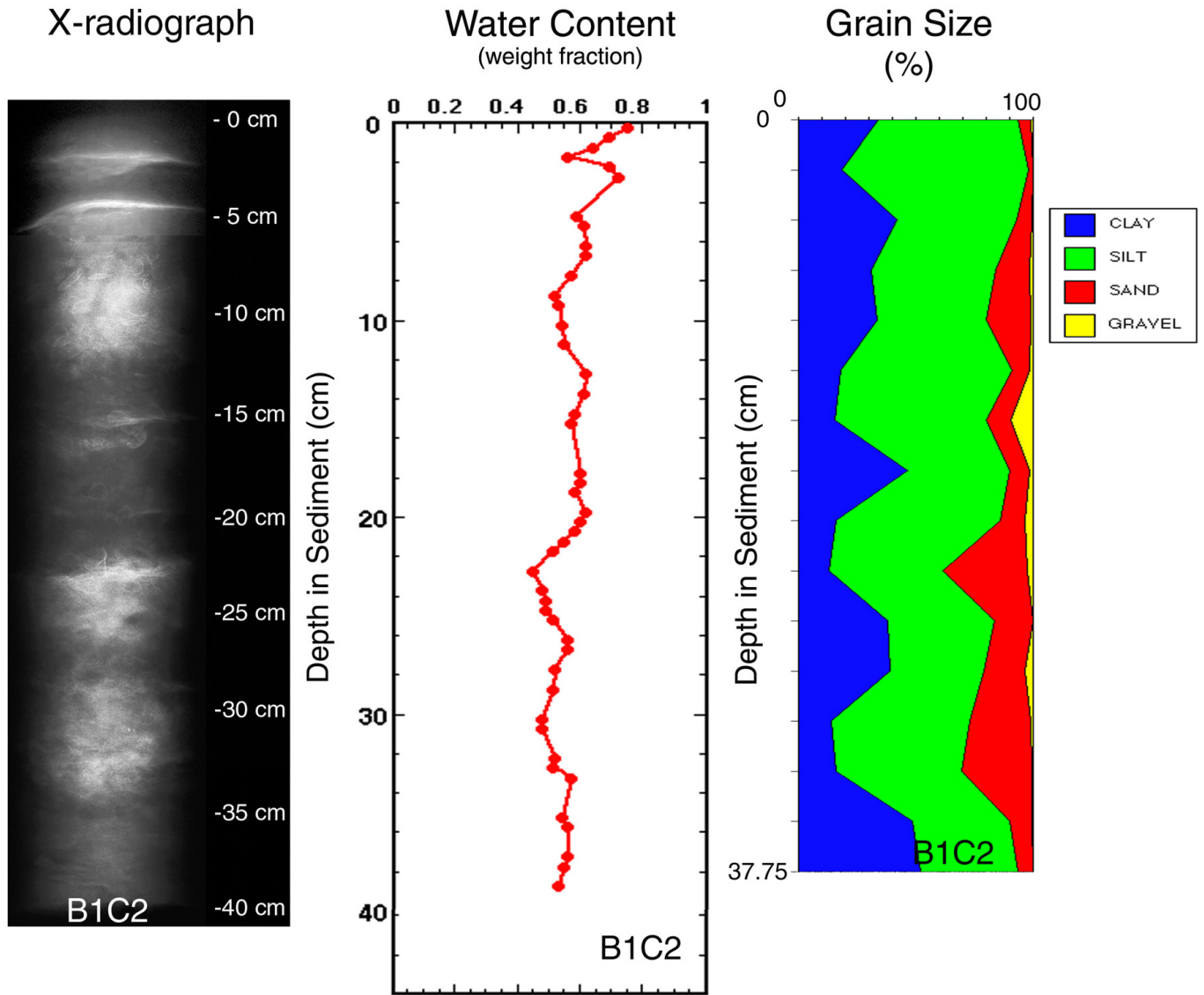
Core B1C2 was taken on June 19, 1996 in 6.5 meters of water. The core measured 39.8 cm in length, was x-rayed on June 26, 1996 and was subsampled on July 30, 1996 at 0.5 cm intervals down the whole core. Features noted are seen in the x-ray, water content, and texture profiles above and include defined sand and mud ribbons, mottled sediment, and abundant biological features such as shell layers.
