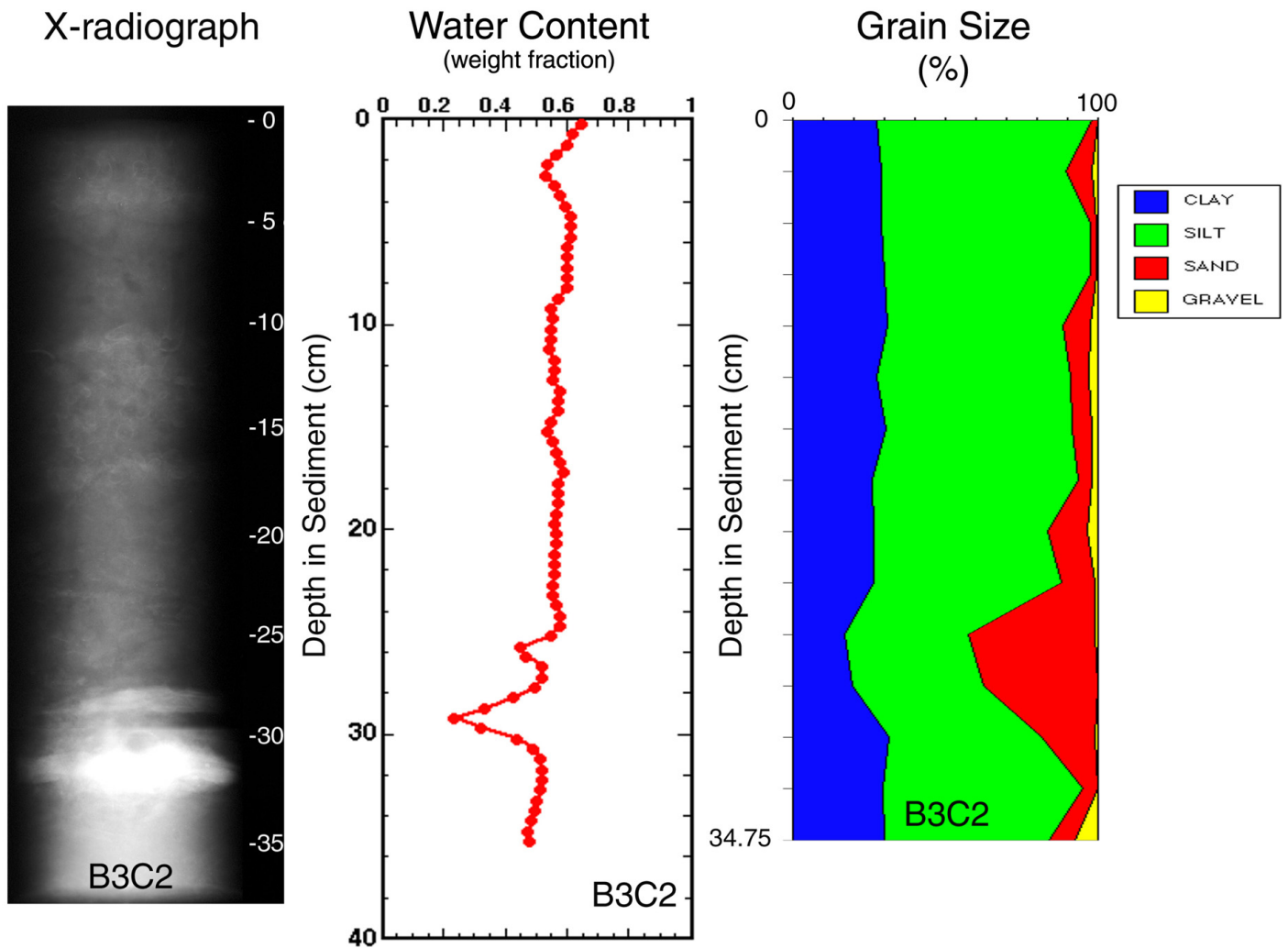
Core B3C2 was taken on June 19, 1996 in 13 meters of water. The core measured 36 cm in length, was x-rayed on June 25, 1996 and was subsampled on October 24, 1996 at 0.5 cm intervals down the whole core. Features noted are seen in the x-ray, water content, and texture profiles above and include sand and mud deposits, mottled sediment, and biological features such as significant shell layers.
