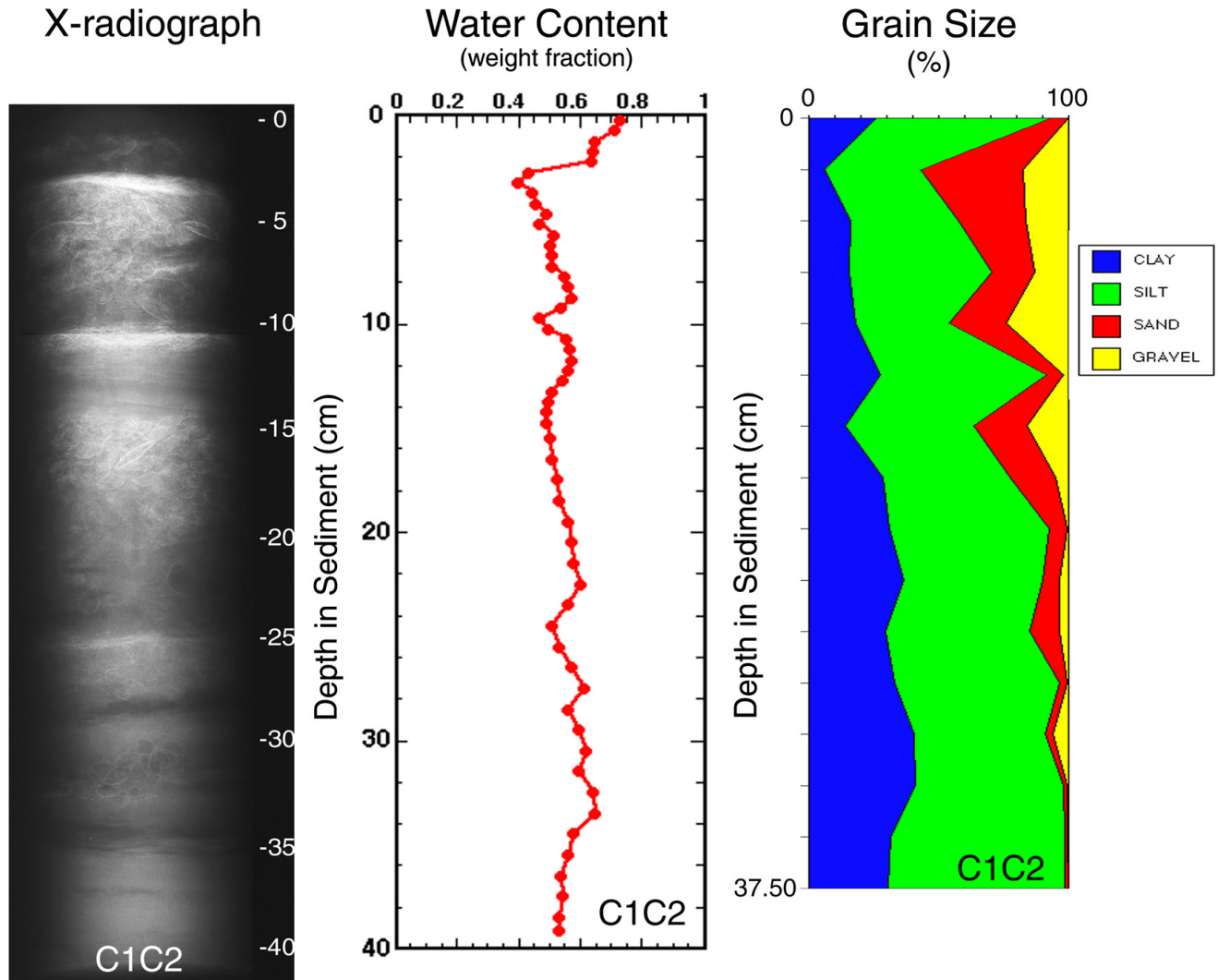
Core C1C2 was taken on June 19, 1996 in 9 meters of water. The core measured 40.1 cm in length, was x-rayed on June 25, 1996 and was subsampled on July 23, 1996 at 0.5 cm intervals down to 15 cm and at 1 cm intervals below 15 cm. Features noted are seen in the x-ray, water content, and texture profiles above and include sand and mud ribbons, and biological features such as abundant shell layers.
