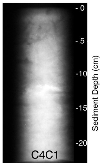
Core C4C1 was taken on June 19, 1996 in 28 meters of water. The core measured 24 cm in length and was x-rayed on June 25, 1996. Features noted are seen in the x-ray above and include mottled sediment, sand and mud deposits, and some biological features such as worm tubes.
