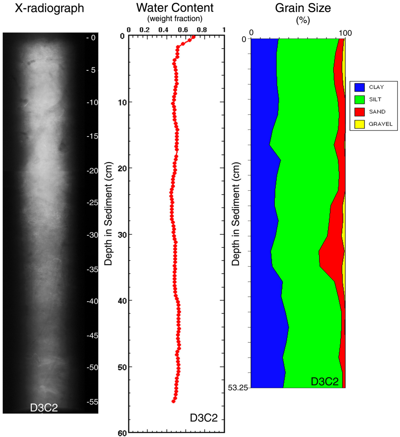
Core D3C2 was taken on June 19, 1996 in 15 meters of water. The core measured 55.4-55.9 cm in length, was x-rayed on June 25, 1996 and was subsampled on October 10, 1996 at 0.5 cm intervals down the whole core. Features noted are seen in the x-ray, water content, and texture profiles above and include mottled sediment and biological features such as shells and worm tubes.
