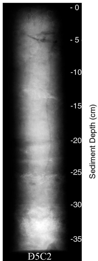
Core D5C2 was taken on June 20, 1996 in 23 meters of water. The core measured 37.5 cm in length and was x-rayed on July 1, 1996. Features noted are seen in the x-ray above and include mottled sediment, wispy sand deposits, and biological features such as small shells and worm tubes.
