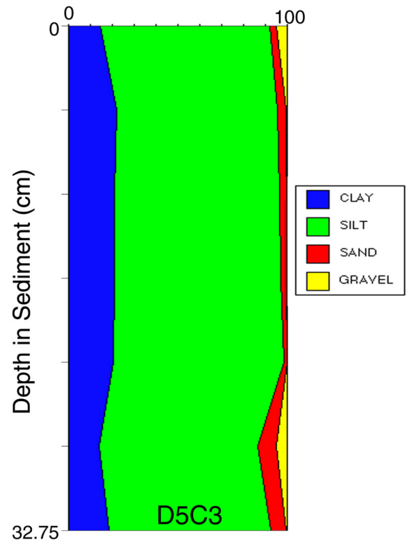
Grain Size (%)
