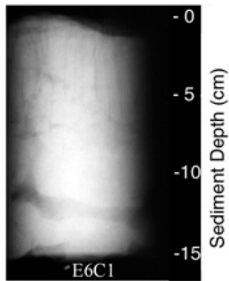
Core E6C1 was taken on June 20, 1996 in 23 meters of water. The core measured 15 cm in length and was x-rayed on July 1, 1996. Features noted are seen in the x-ray above and include mottled sediment, gas, and some biological features such as worm tubes.
