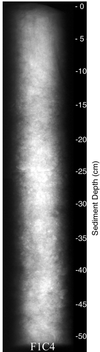
Core F1C4 was taken on June 20, 1996 in 9 meters of water. The core measured 51.5-52.5 cm in length and was x-rayed on July 2, 1996. Features noted are seen in the x-ray above and include mottled sediment and some biological features such as small shells and worm tubes.
