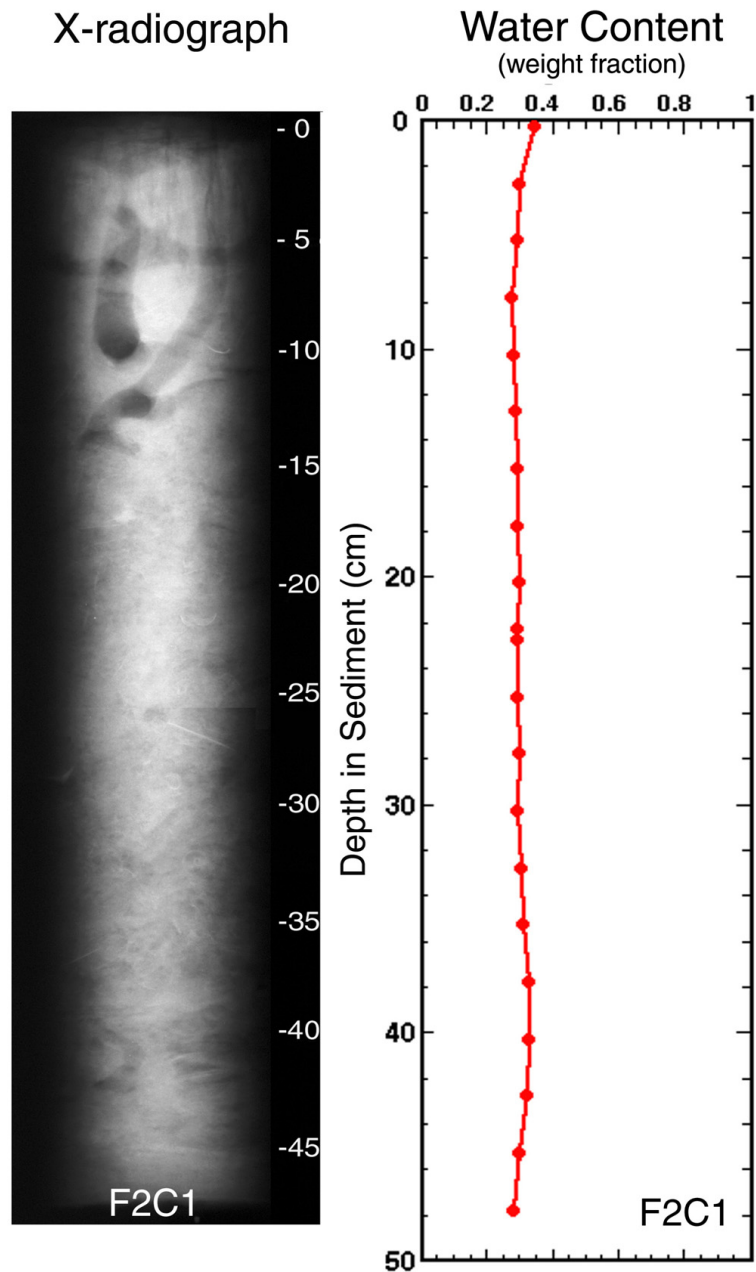
Core F2C1 was taken on June 20, 1996 in 9 meters of water. The core measured 48 cm in length, was x-rayed on July 2, 1996 and was subsampled on June 16, 1998 at 0.5 cm intervals down the whole core. Features noted are seen in the x-ray and water content profiles above and include mottled sediment, wispy sand deposits, and some biological features such as small shells and worm tubes. No textural analysis is intended for this core.
