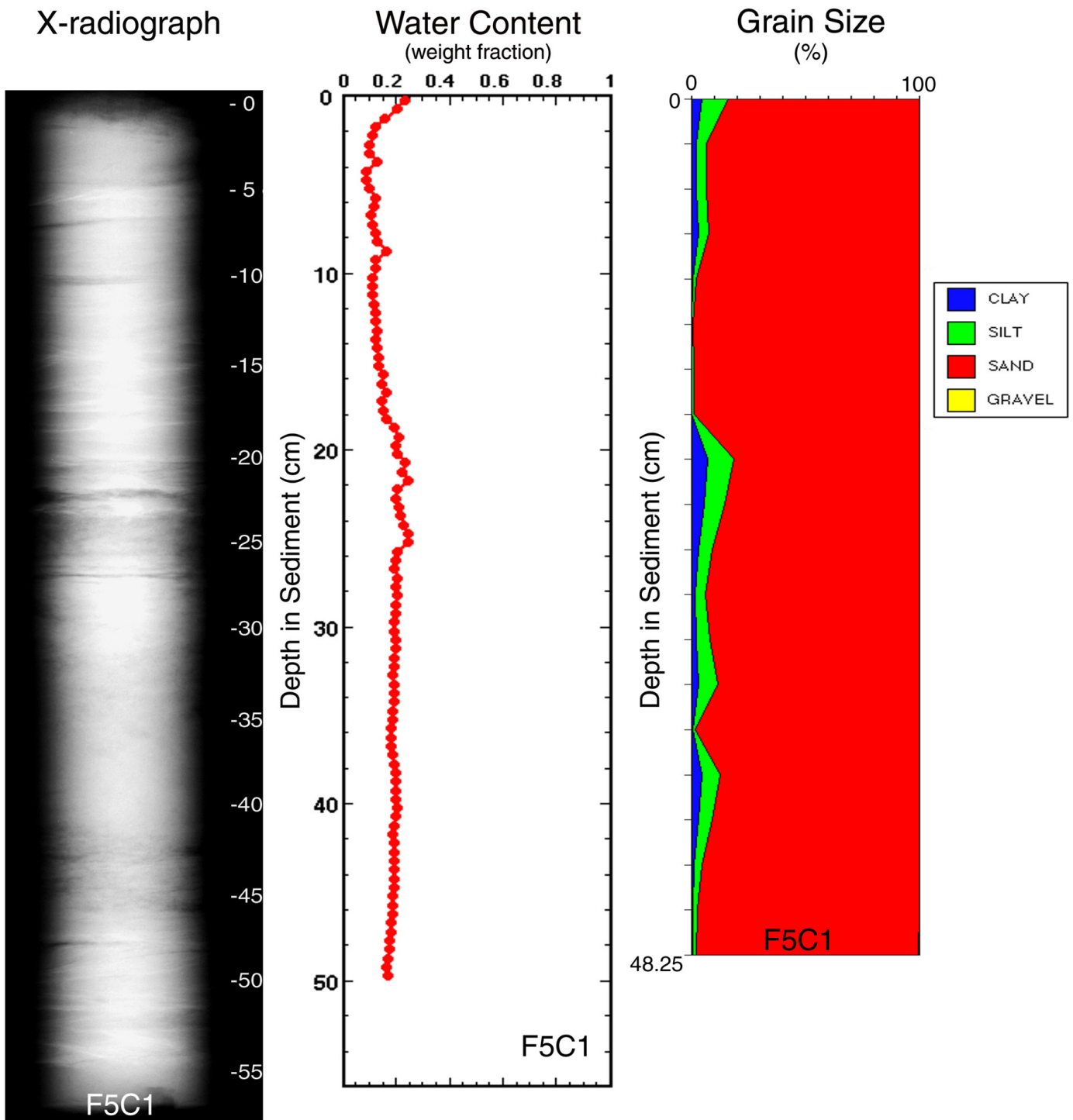
Core F5C1 was taken on June 20, 1996 in 34 meters of water. The core measured 55.4-55.8 cm in length, was x-rayed on July 2, 1996 and was subsampled on February 3, 1997 at 0.5 cm intervals down the whole core. Features noted are seen in the x-ray, water content, and texture profiles above and include sand and mud ribbons and some mottled sediment.
