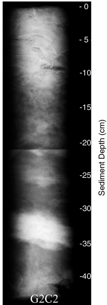
Core G2C2 was taken on June 21, 1996 in 15 meters of water. The core measured 43.5 cm in length and was x-rayed on July 1, 1996. Features noted are seen in the x-ray above and include mottled sediment, wispy angled sand deposits, and some biological features such as shells.
