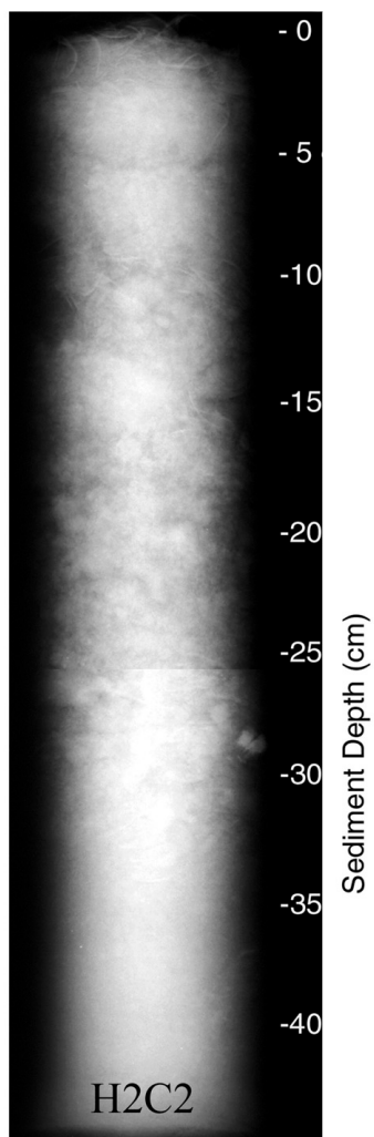
Core H2C2 was taken on June 21, 1996 in 38 meters of water. The core measured 44 cm in length and was x-rayed on July 1, 1996. Features noted are seen in the x-ray above and include mottled sediment and some biological features such as shells, especially in the top 5 cm.
