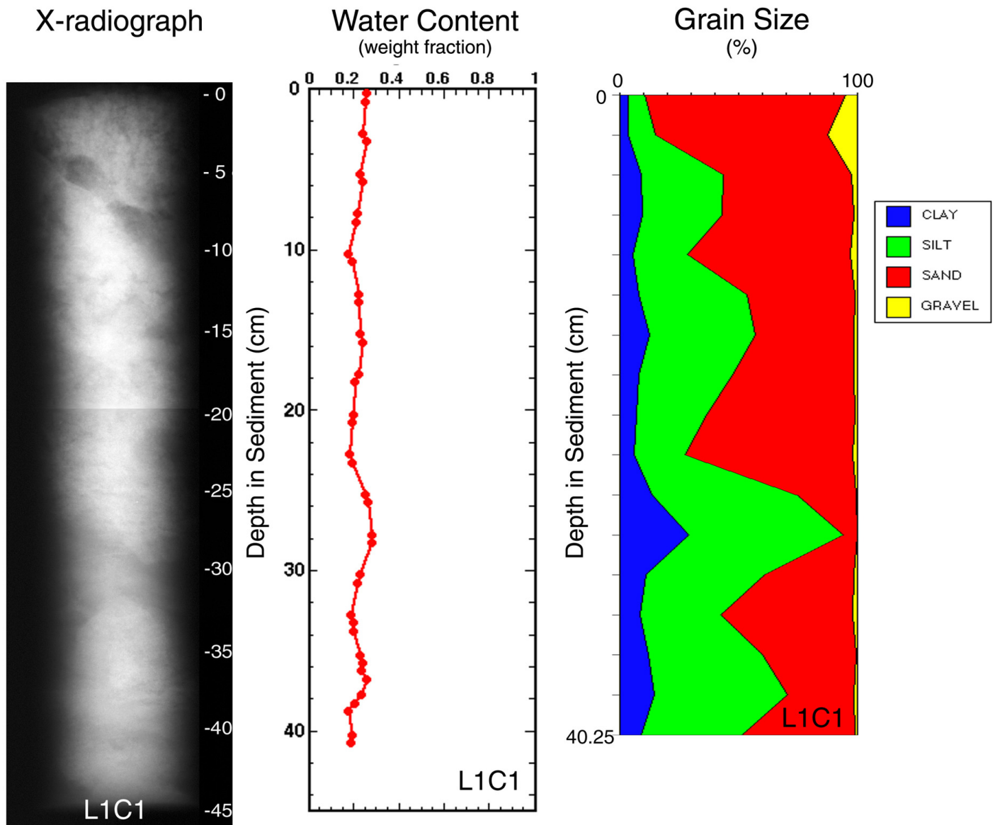
Core L1C1 was taken on June 21, 1996 in 40 meters of water. The core measured 44.5 cm in length, was x-rayed on July 1, 1996 and was subsampled on September 25, 1996 at 0.5 cm intervals down the whole core. Features noted are seen in the x-ray, water content, and texture profile above and include angled deposits, mottled sediment, and some biological features.
