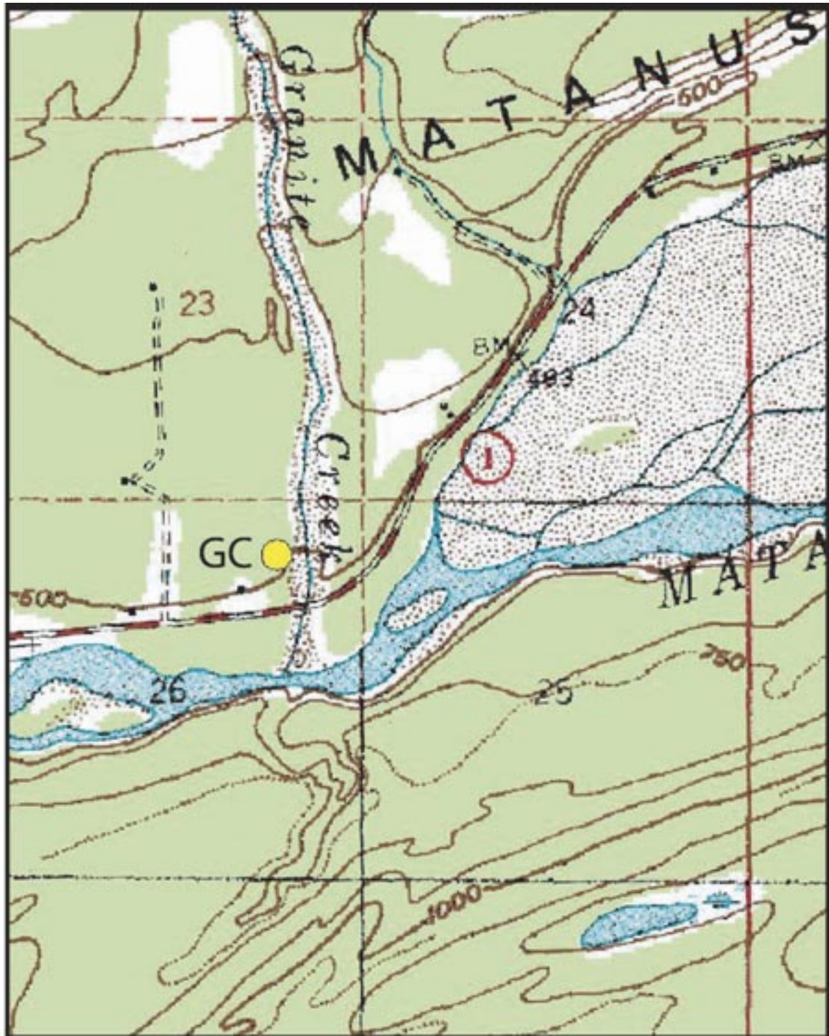
Detail of the Anchorage C-5 Quadrangle, showing the location of the Granite Creek field site. This site samples boulders from a variety of source formations in the Granite Creek stream bed, just off of the Glenn Highway 14 miles northeast of Palmer.
