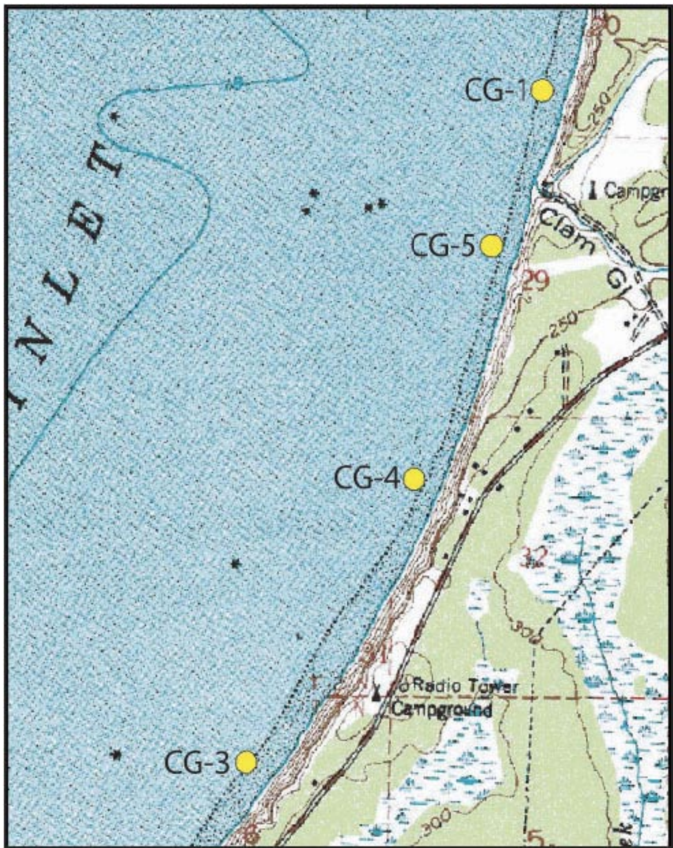
Detail of Kenai A-4 Quadrangle, showing the location of Clam Gulch field sites 1, 3, 4 and 5. These sites sample the Sterling Formation where it is exposed in the sea cliffs near Clam Gulch.
