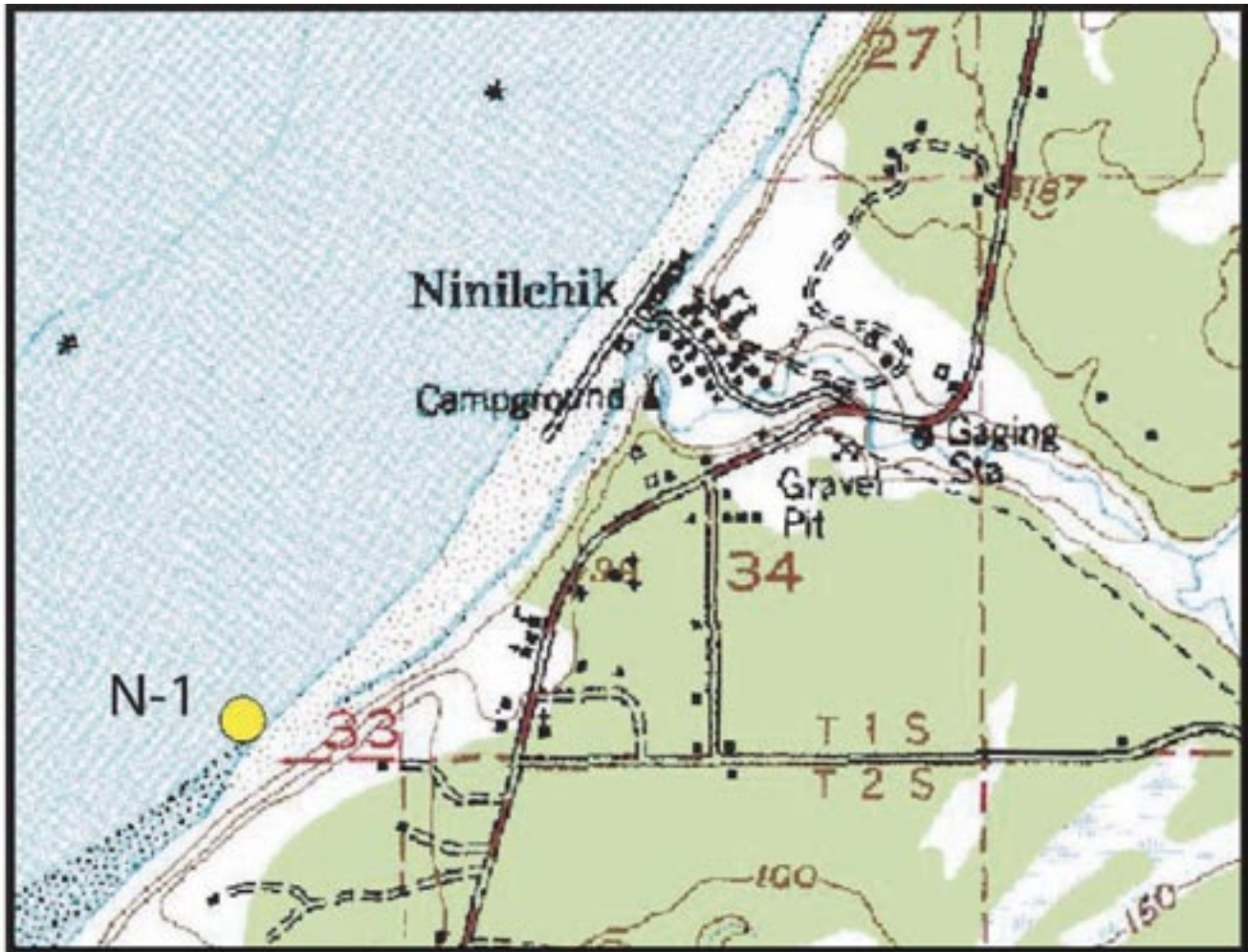
Detail of the Kenai A-5 Quadrangle, showing the location of the Ninilchik field location. This site samples the Sterling Formation where it is exposed in the sea cliffs southwest of Ninilchik.
