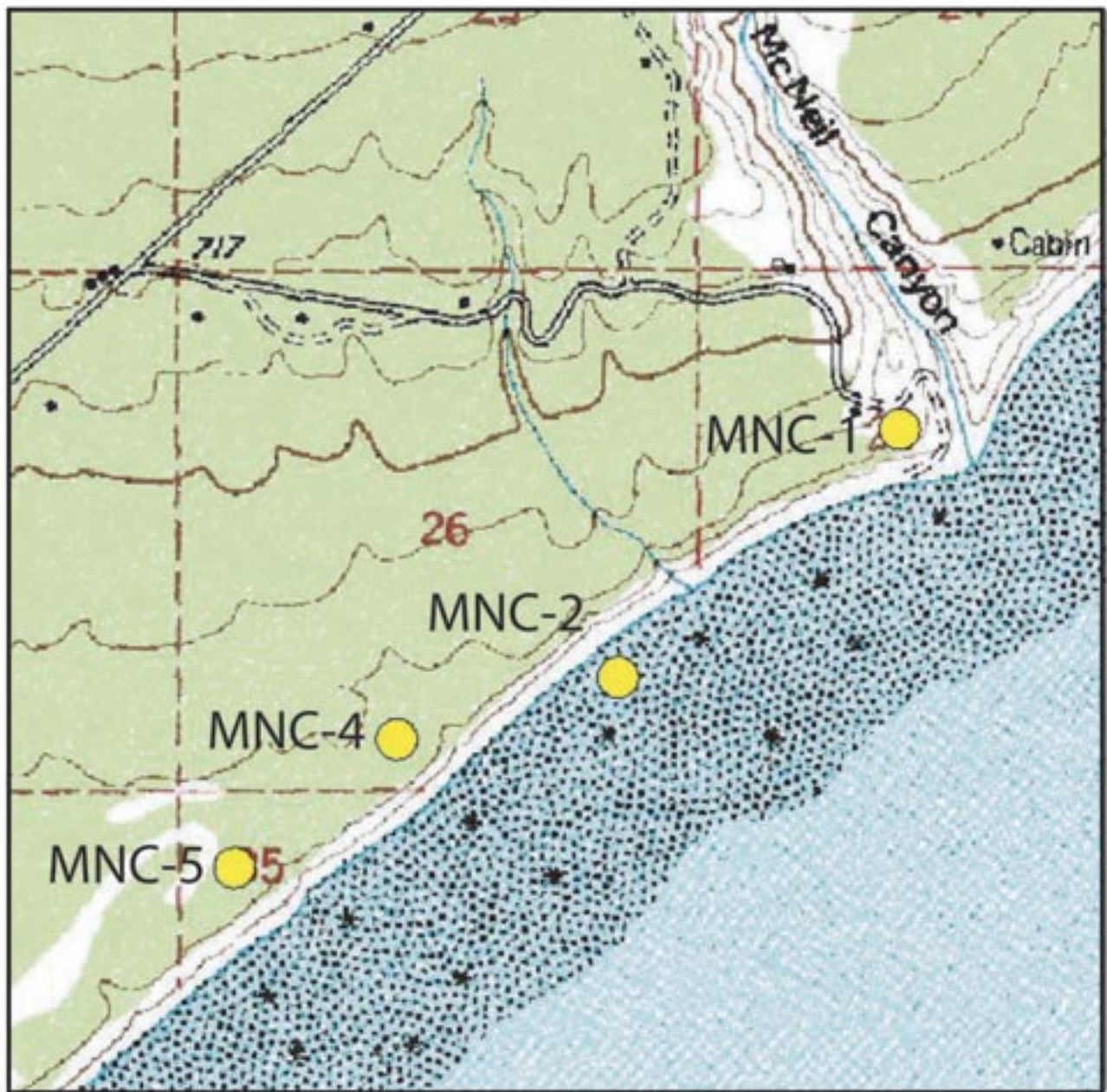
Detail of the Seldovia C-4 Quadrangle, showing the locations of McNeil Creek field sites 1-5. These localities sample the Beluga Formation where it is exposed in the sea cliffs northwest of Homer.
