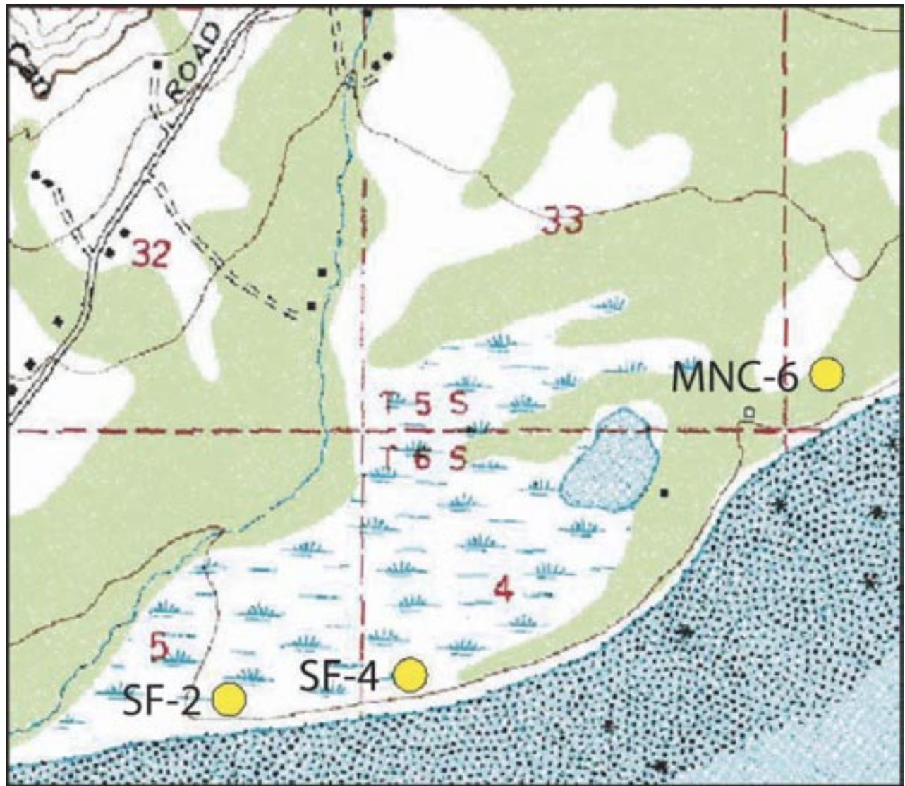
Detail of the Seldovia C-4 Quadrangle, showing the locations of Sea Side Farms field sites 2 and 4, McNeil Creek field site 6. These localities sample the Beluga Formation where it is exposed in the sea cliffs northeast of Homer.
