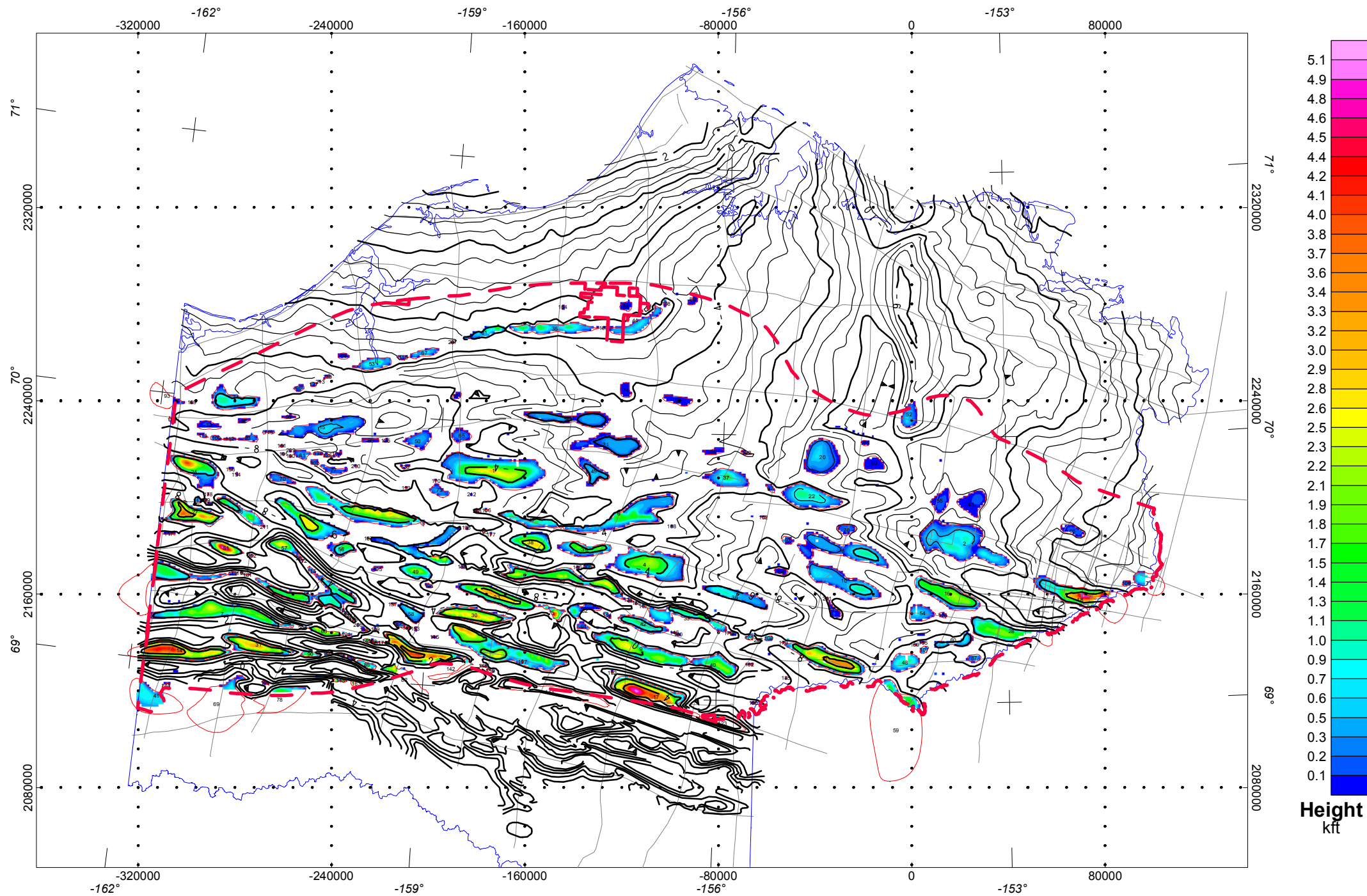
Closure Map - Brookian Topset Structural Play - Nanushuk Horizon Tetra Tech 400-550 horizons with datum shifts to TT 500 27 February 2002
