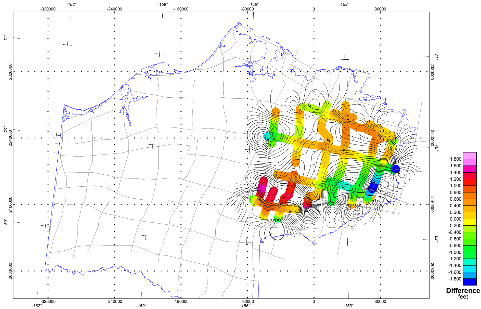
Depth Differences in Tetra Tech vs USGS Seismic Mapping Tetra Tech 1400 minus USGS Endicott USGS NPRA Project
