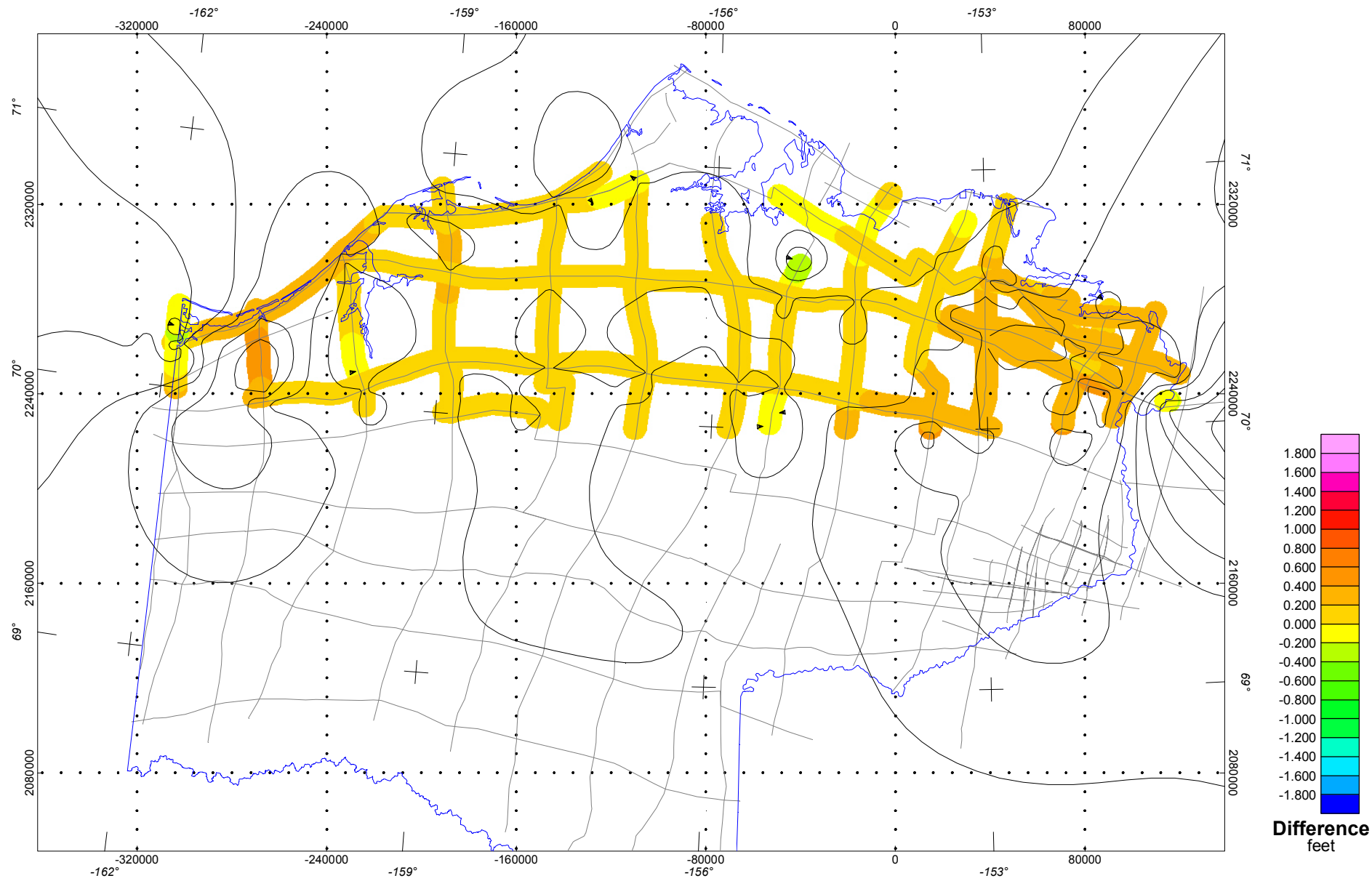
Depth Differences in Tetra Tech vs USGS Seismic Mapping Tetra Tech 1040 minus USGS Sadlerochit USGS NPRA Project
