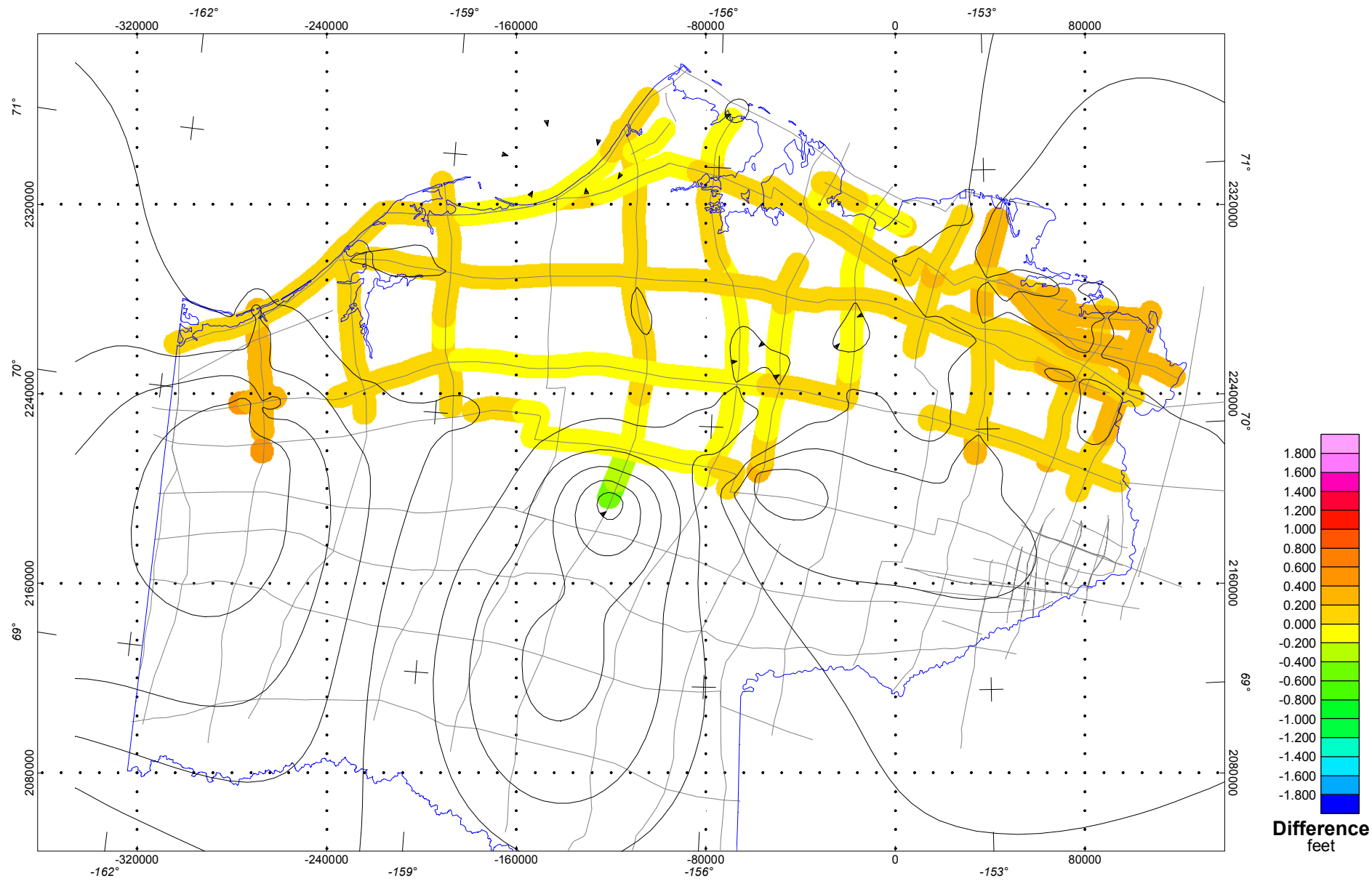
Depth Differences in Tetra Tech vs USGS Seismic Mapping Tetra Tech 1000/1020 minus USGS Sag River USGS NPRA Project
