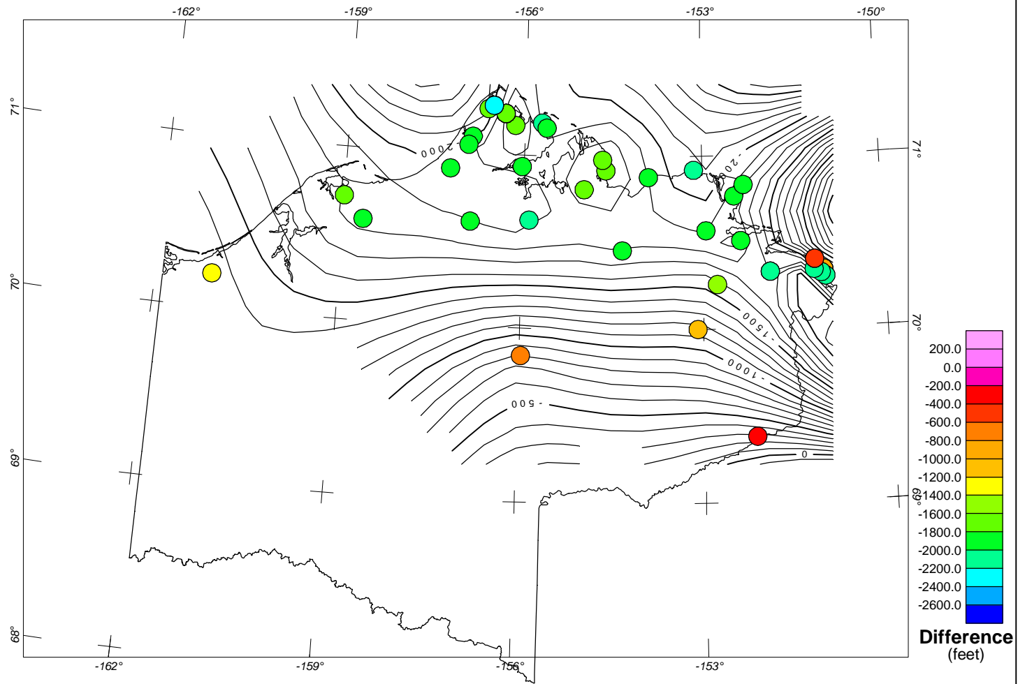
LCU differences Well depths - seismic depths Saltus 26 Feb 2002
