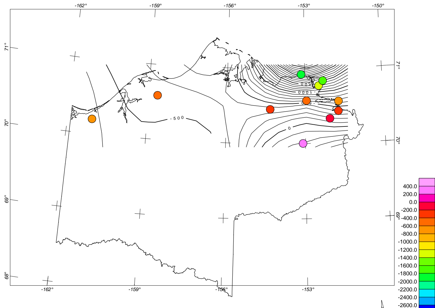
LIS differences Well depths - seismic depths Saltus 26 Feb 2002
