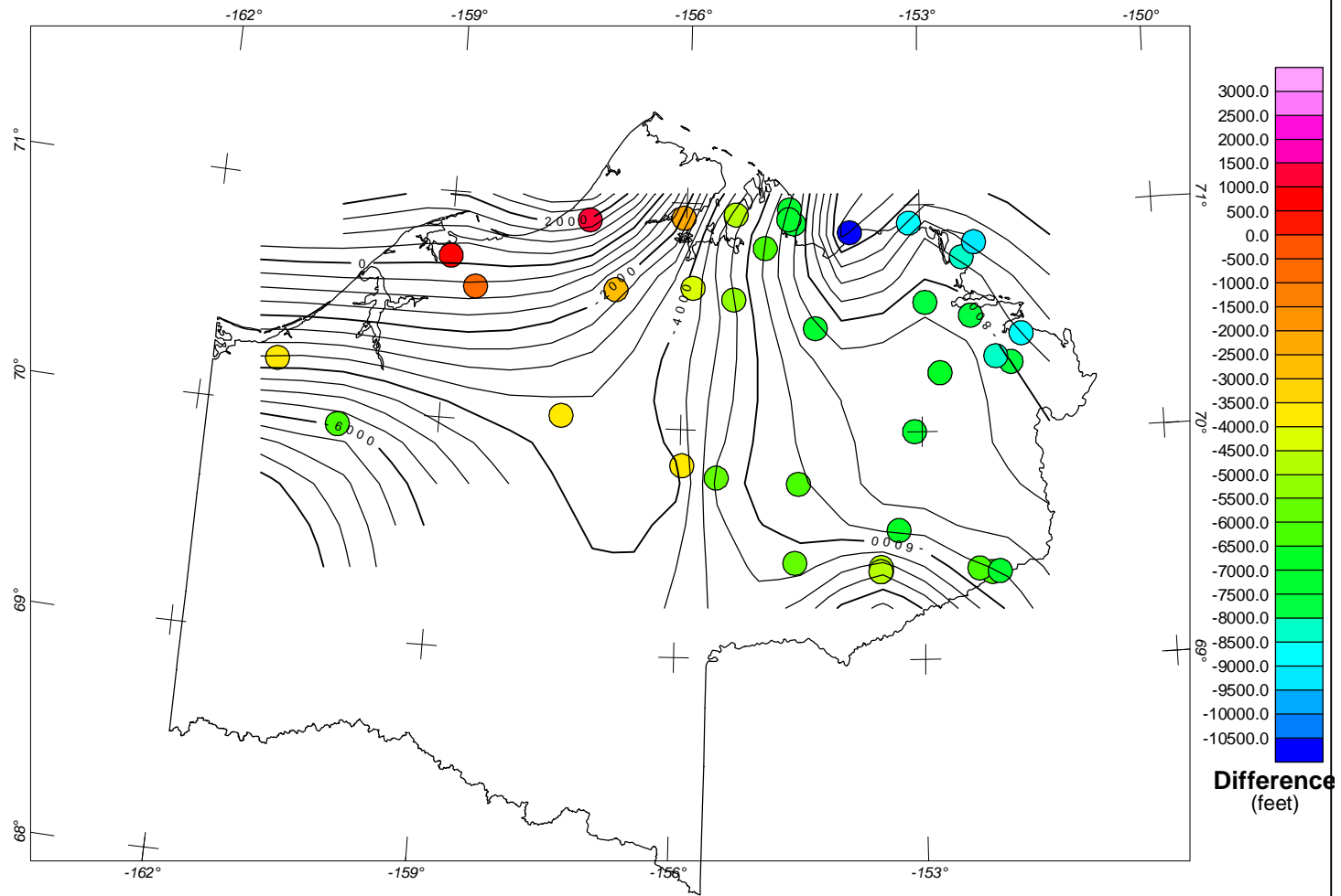
NNU differences Well depths - seismic depths Saltus 26 Feb 2002
