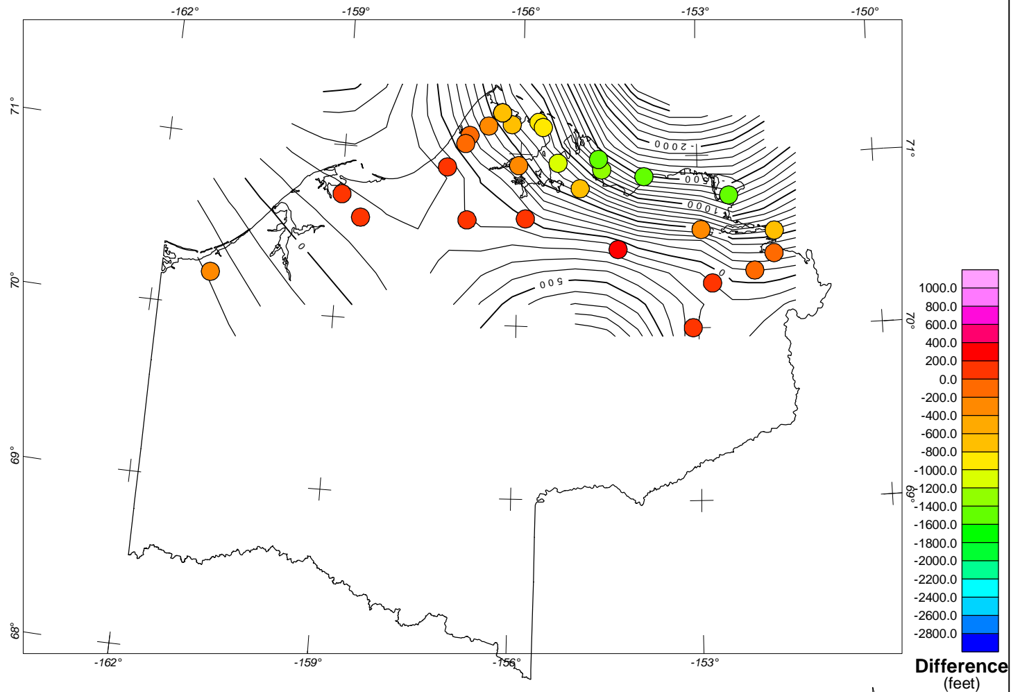
SAG differences Well depths - seismic depths Saltus 26 Feb 2002
