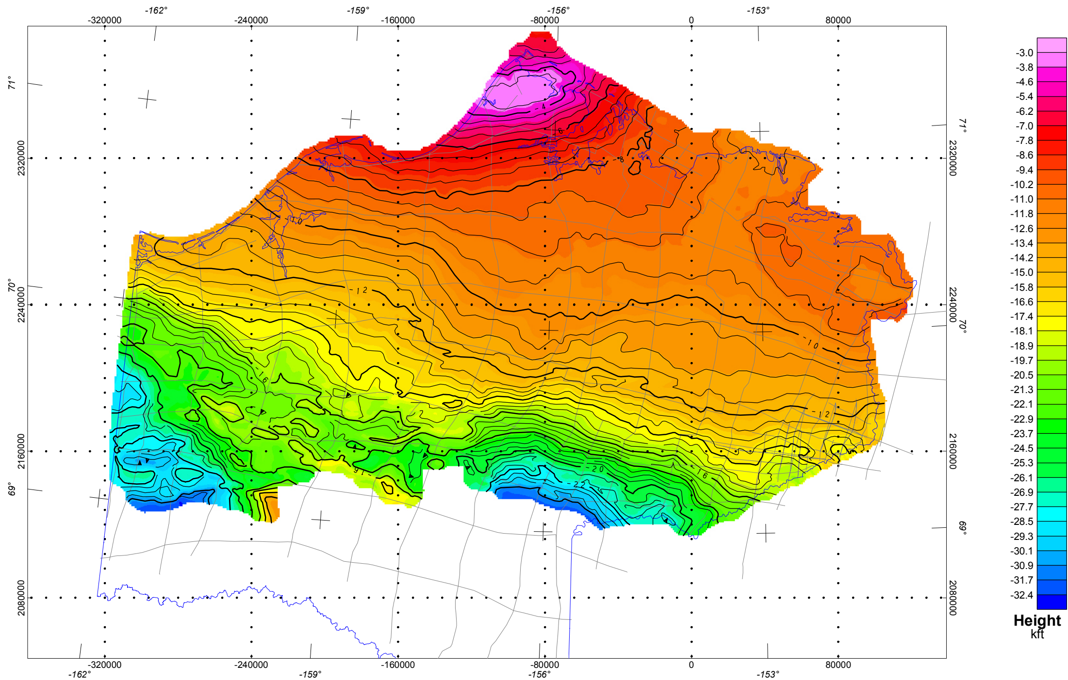
Horizon - LCU Tetra Tech 700/720 with USGS corrections 12 December 2001
