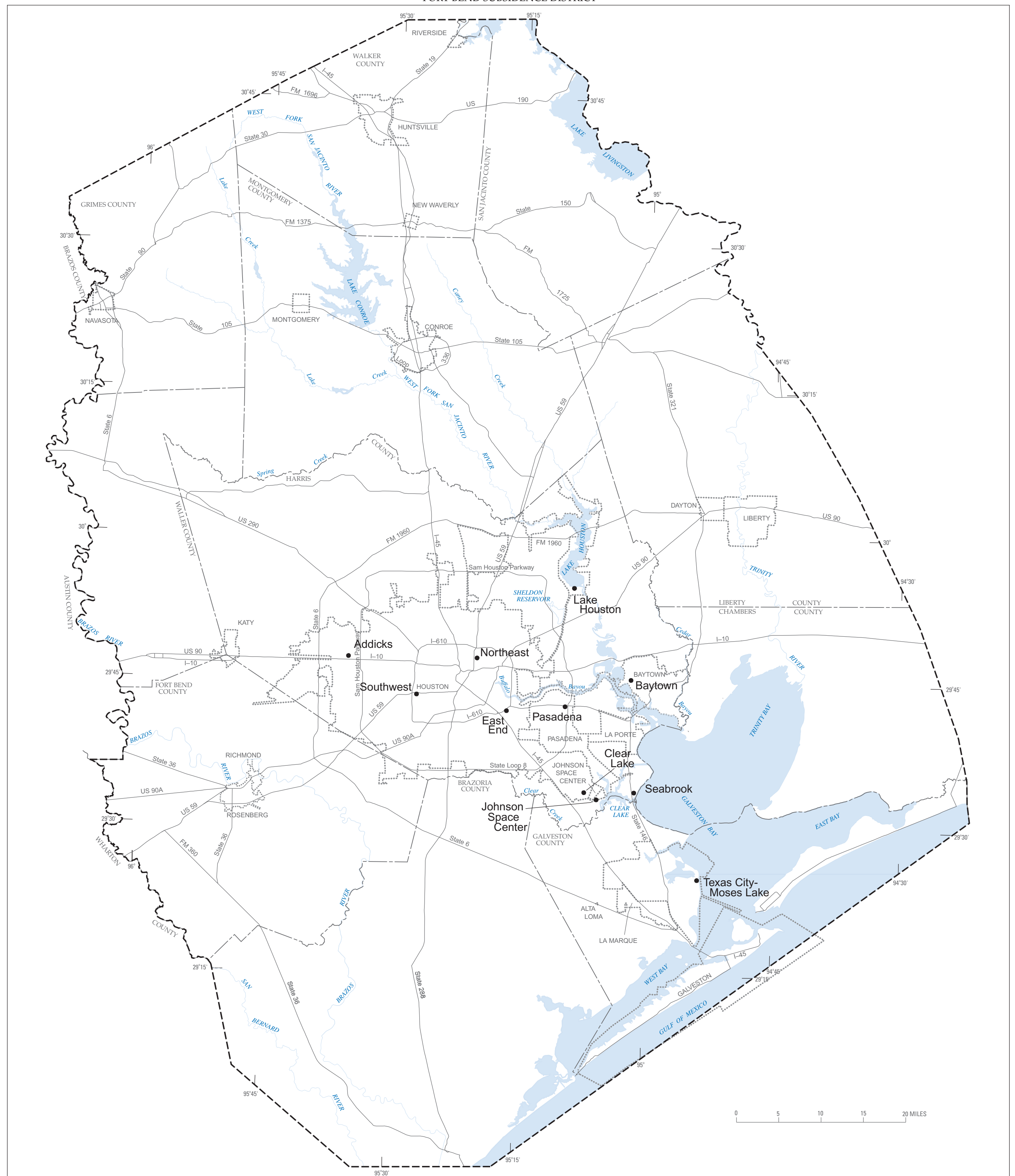
Figure 14. Map showing location of extensometer sites, Houston-Galveston region, Texas.
