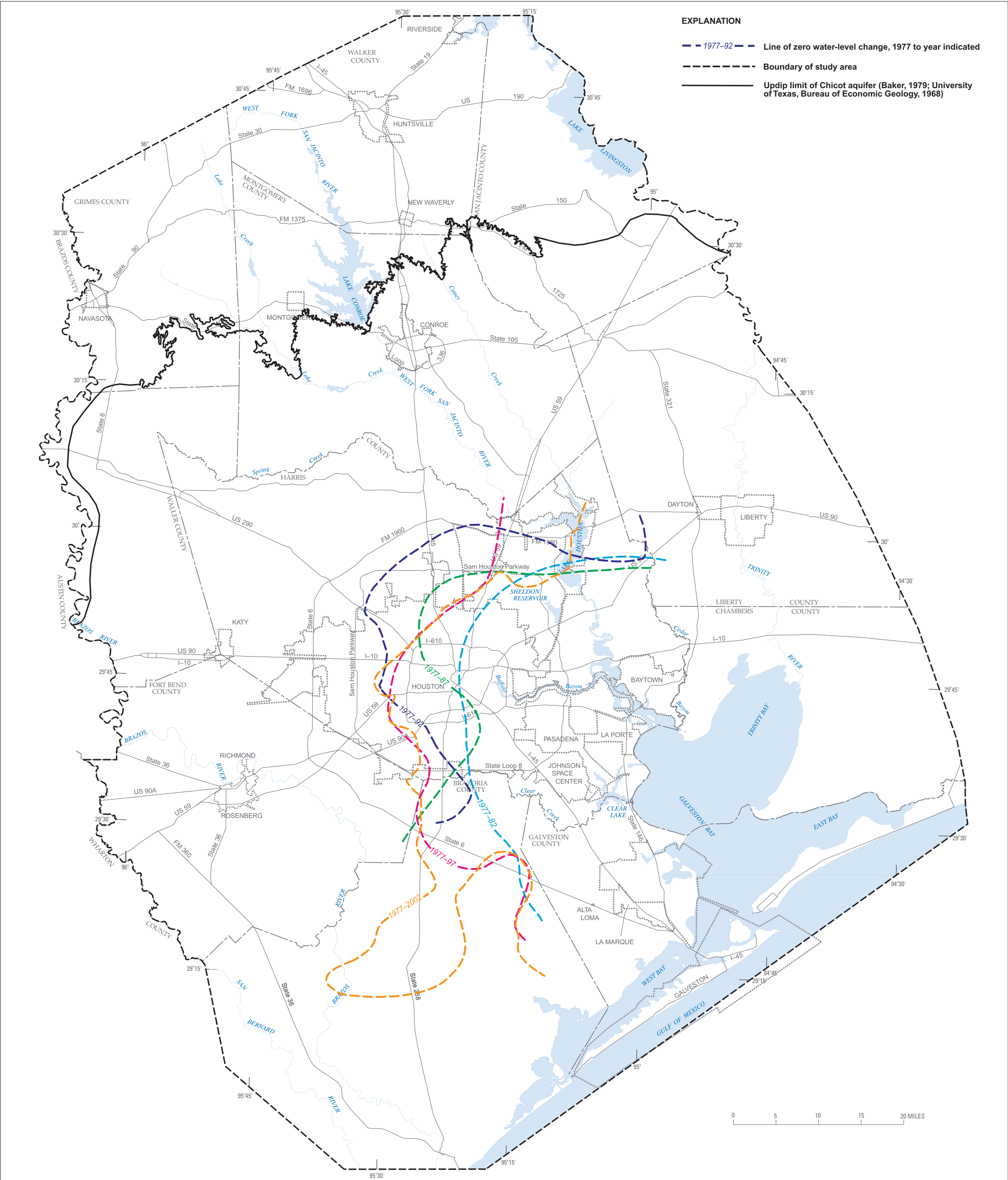
Figure 4. Map showing lines of zero water-level change in the Chicot aquifer, Houston-Galveston region, Texas, for intervals increasing in 5-year increments beginning with 1977-82.
