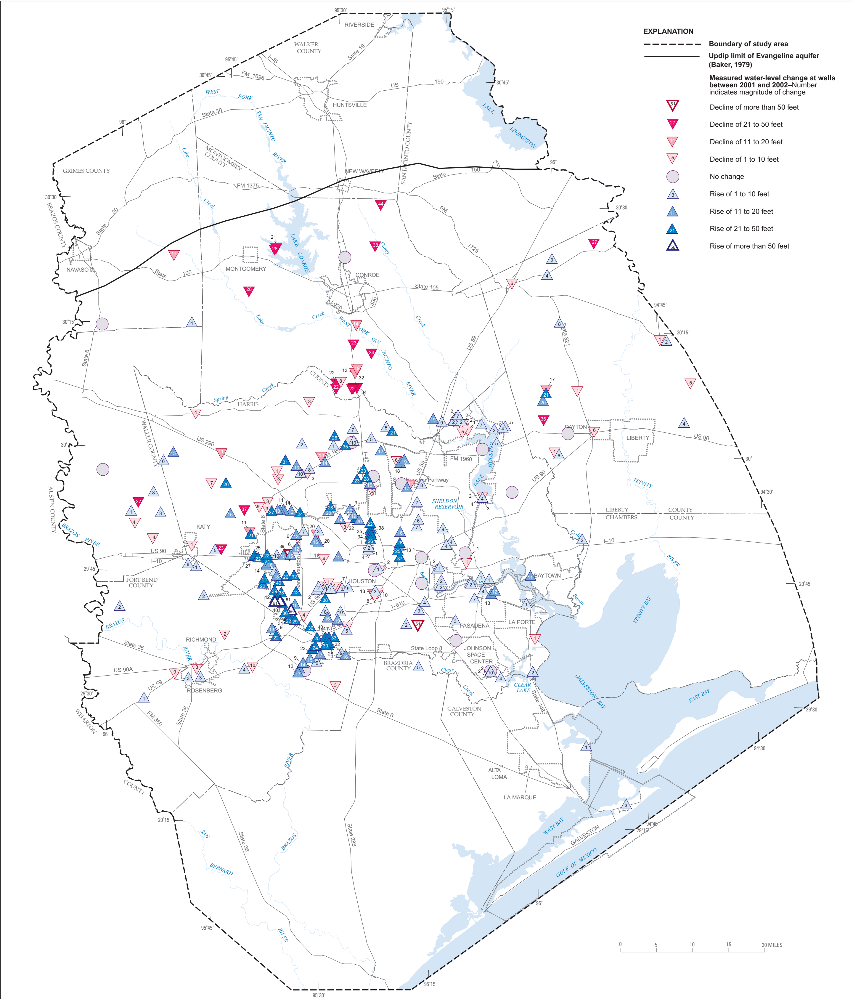
Figure 7. Map showing water-level changes in the Evangeline aquifer, Houston-Galveston region, Texas, 2001-02.
