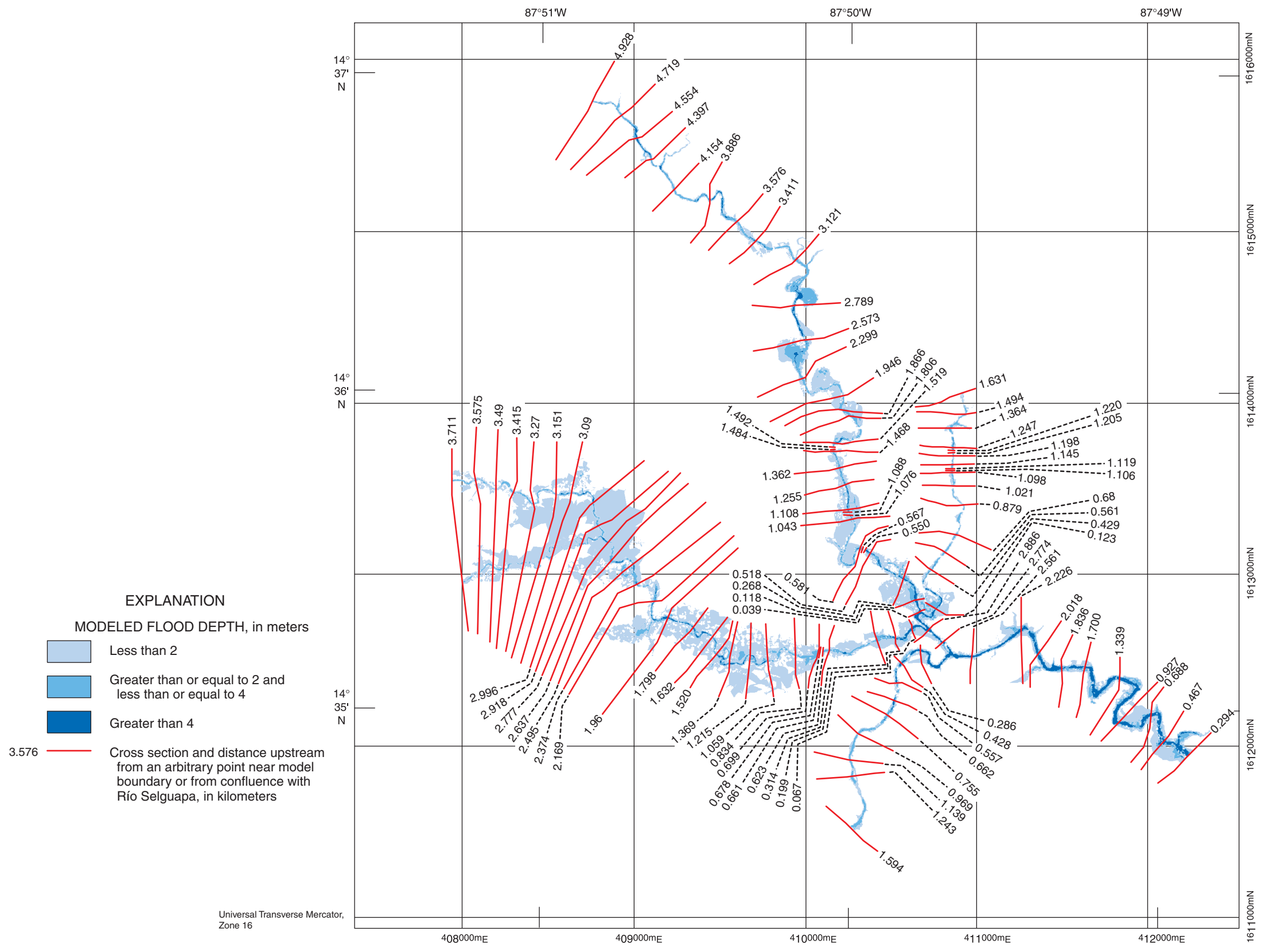
Figure 7. Depth of inundation for the 50-year flood and location of cross sections on Río Selguapa, Río Guique, Río Celan, Río Calan, and Quebrada Chalantuma at Siguatepeque, Honduras.
