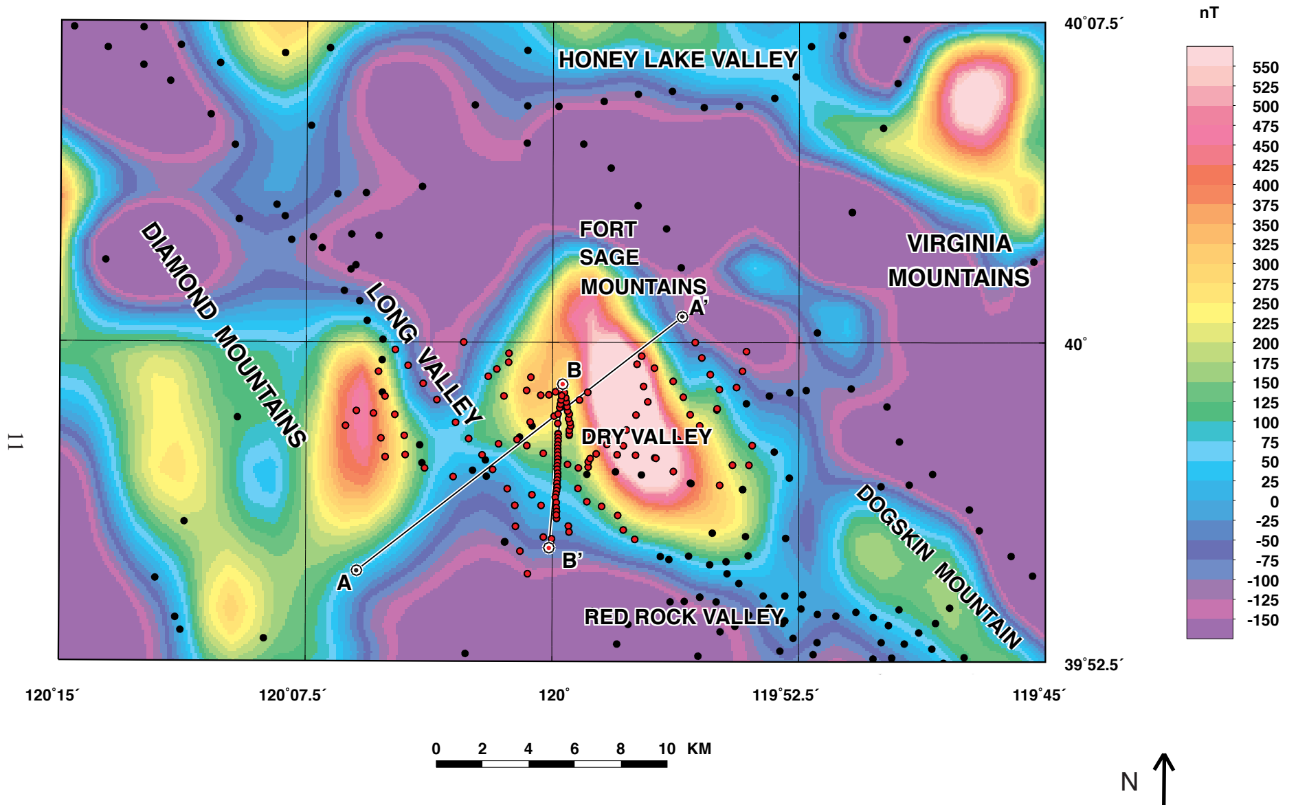
Figure 5. Aeromagnetic map of the study area (modified from Hildenbrand and Kucks, 1988). See figure 2 for explanation.
