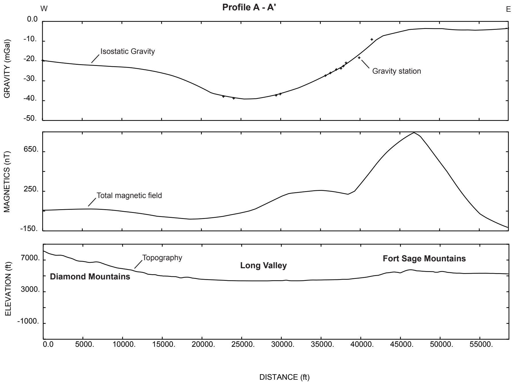
Figure 6. Isostatic gravity, magnetic, and topographic profiles across Long Valley. Crosses, scattered gravity stations along the profile. Vertical exaggration = 1.
