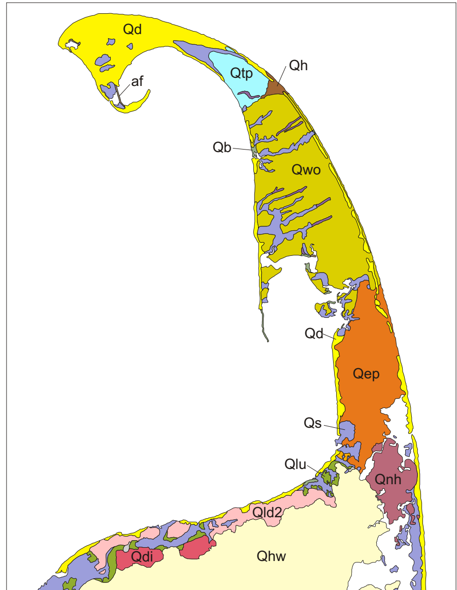
Figure 3. Surficial geologic map and correlation of geologic units of Lower Cape Cod (from Oldale and Barlow, 1986). See figure 4 for place names and town boundaries.
