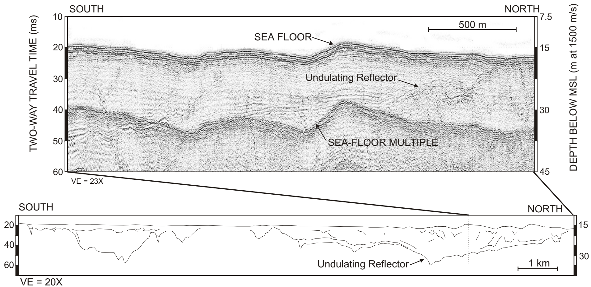
Figure 5. Interpretive cross section and section of Boomer seismic profile located east of Orleans and Eastham (see Fig. 4 for profile location). Undulating reflector is the same horizon mapped by Aubrey and others (1982).
