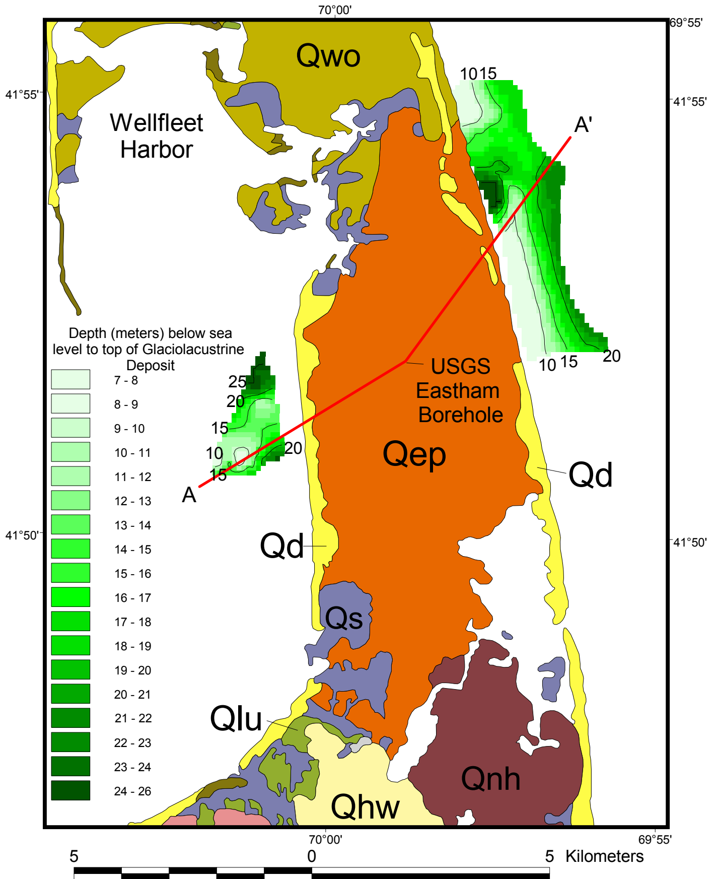
Figure 8. Map showing the depth (meters) to the surface of glaciolacustrine (Qdl). Cross-lined area indicates area where the Holocene transgression has eroded Qdl. Location of cross section A (Fig. 13) shown by red line. Surficial geologic units are described in figure 3.
