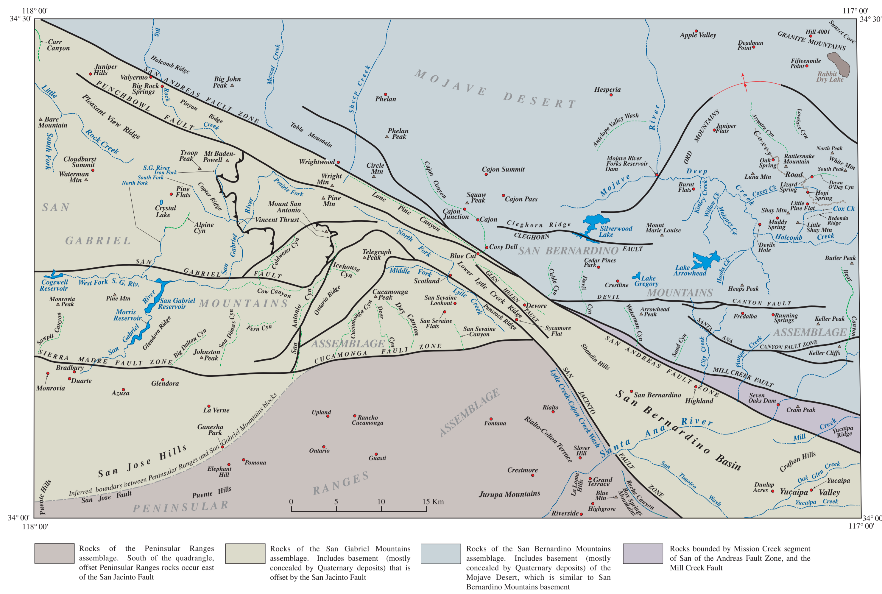
Figure 1. Map of San Bernardino 30' X 60' quadrangle showing place names used in Description of Map Units, Regional Synthesis, and Geologic Notes. Colored areas define structural assemblages. Approximate locations of most faults having large displacements or lengths are shown. Inferred boundary between Peninsular Ranges and San Gabriel Mountains assemblages is hidden beneath thick Quaternary deposits, and its location and character are highly speculative. Town or geographic feature, Mountain Peak.
