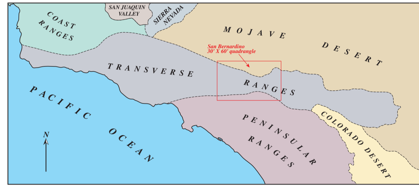
Figure 2. Map showing San Bernardino 30' X 60' quadrangle in relation to physiographic provinces in southern California. Within the quadrangle, provinces and province boundaries do not conform to the rock assemblages designated in the geologic notes accompanying the DESCRIPTION OF MAP UNITS.
