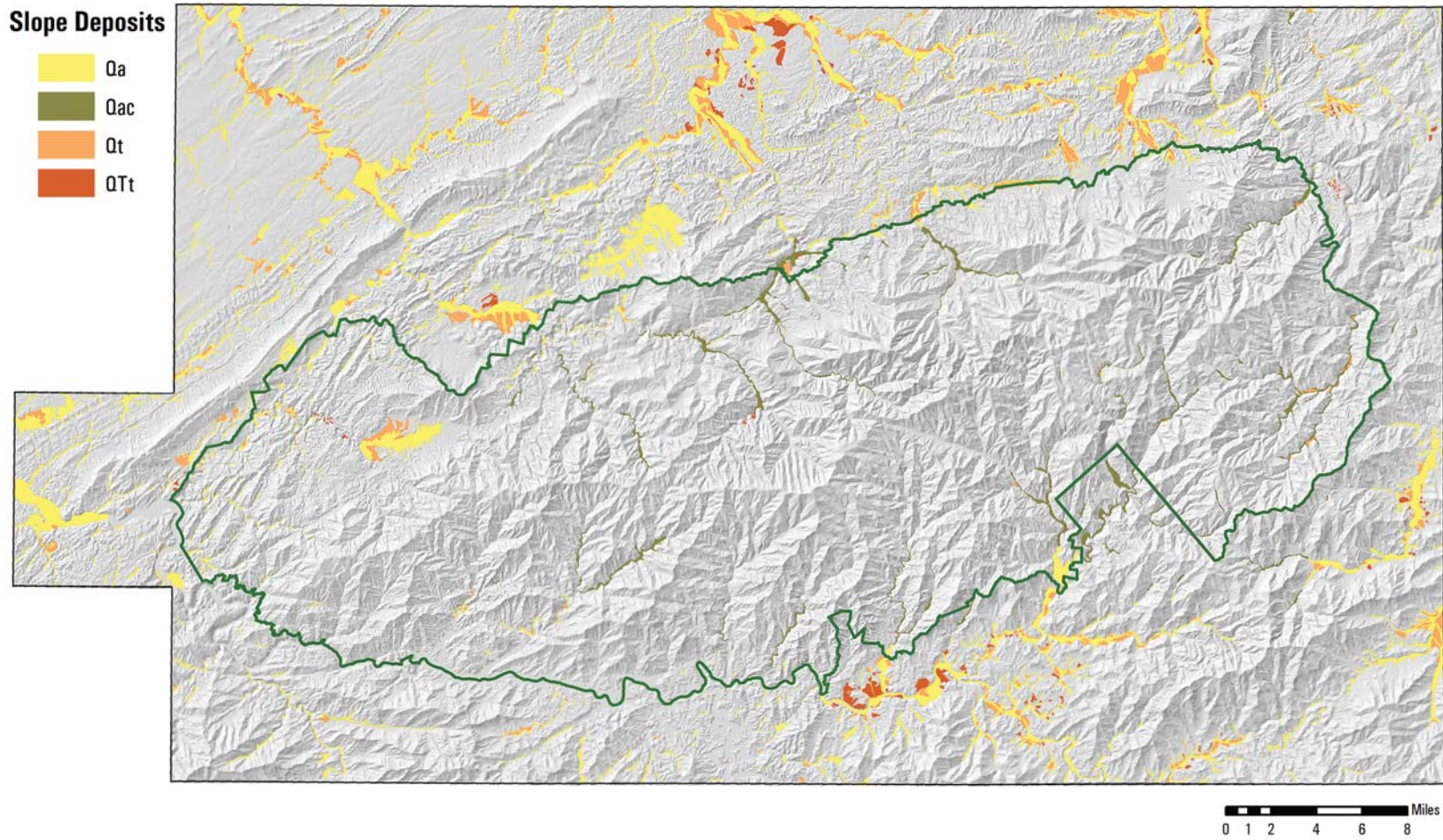
Fig. 12- Distribution of alluvium, coarse alluvium, and terraces within the study area are shown on a digital elevation model hillshade.
