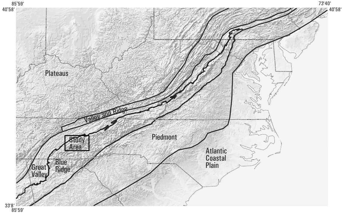
Fig. 2- A) Physiographic provinces of the Appalachian region.
